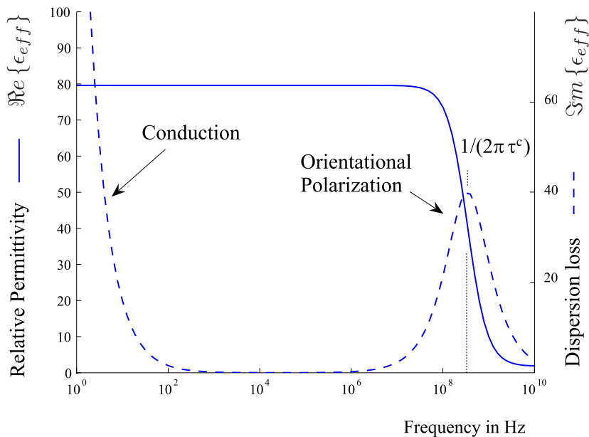
FIG. 10.2 – Graphical representation of the real part of the dielectric constant ( \epsilon' full line) and the imaginary part of the effective conductivity of water ( \Im m\{\epsilon_{eff}\} dashed line). The relaxation time \tau^c can be as small as 4.7 \cdot 10^{-10} s when the water is linked to phospholipidic head groups [127], but normally this one is in the order of 8.27 \cdot 10^{-12} s (for water at 25^\circ [15]). The variation of \epsilon' from 78.8 ( \omega = 0 ) to 1.8 ( \omega = \infty ) is called dielectric decrement. the imaginary part amplitudes where calculated using the Kramers-Kronig implementation of CST. The conductivity at low frequencies is added to the Debye dispersion model, whose relaxation constant is given here. In the range of frequencies where NMR takes place, the dispersion is mostly caused by the rotational motions of the electrically polarized water molecules.
