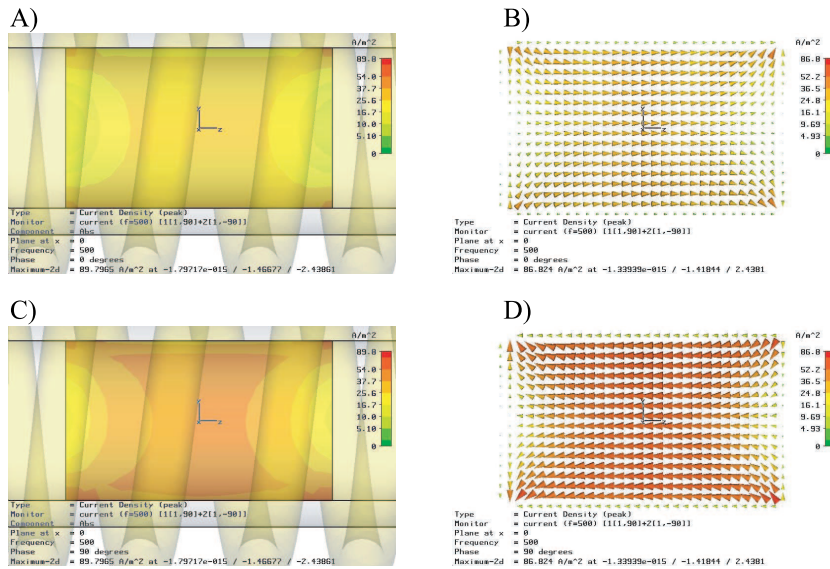
FIG. 10.4 – Current density, calculated inside the lossy water sample. The simulation was done with CST on the already introduced 4 mm variable pitch coil. The sample is a cylinder of 5 mm length and 3 mm in diameter. It is contained in a non-lossy ceramic cylinder of 18 mm of length and 4 mm of outer diameter representing the ZrO_2 rotor. Since the field is polarized it is treated as a complex, whose time phase is to be considered. The first line corresponds to a phase reference, the second is quadrature shifted. The left column corresponds to the so called ‘absolute’ (abs) value of the field, this is a sum of spacial components (X,Y,Z). (A) is ‘abs’ at 0^\circ and (C) the same at 90^\circ . The right columns gives the corresponding distribution as a vector field.
