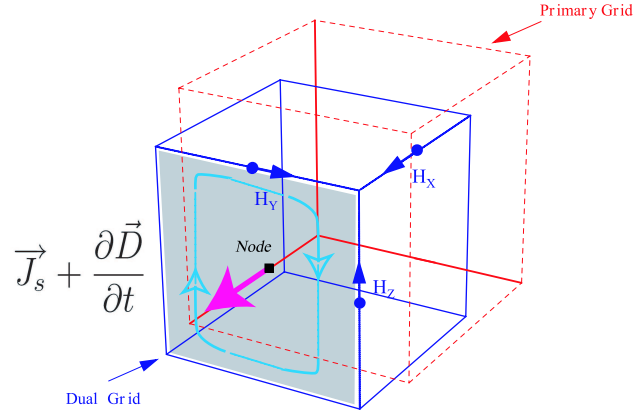
FIG. 4.2 – Loops of magnetic field used to derive currents.
