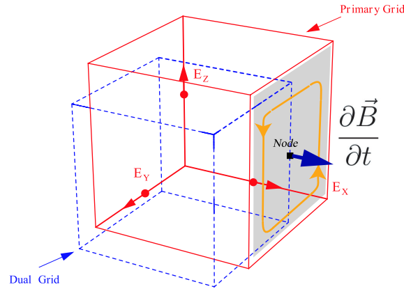
FIG. 4.3 – Circulation of the Electric field in order to derive the flux \Phi .
