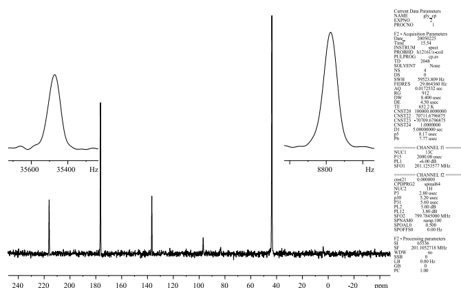
FIG. 11.11 – Sensitivity measurement on the ^{13}\text{C} nucleus of a natural abundance glycine sample packed in a full 4 mm rotor (110 mg). The ^{13}\text{C} CP as been adjusted to a 40 kHz field during the contact pulse (2 ms), for the 1H decoupling SPINAL64 at 90 kHz was employed during 17 ms. The S/N was measured for C- \alpha , using the function 'Sinocal' with 10 ppm noise interval, it yields at 95 :1. The rotation frequency is 8 kHz.
