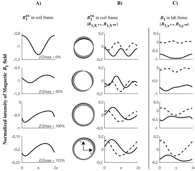
FIG. 8.4 – Set of figures \rho = 1.5 \text{ mm} : Magnetic field vectors calculated in the empty coil, and displayed around circular rings of diameter 3 mm.
