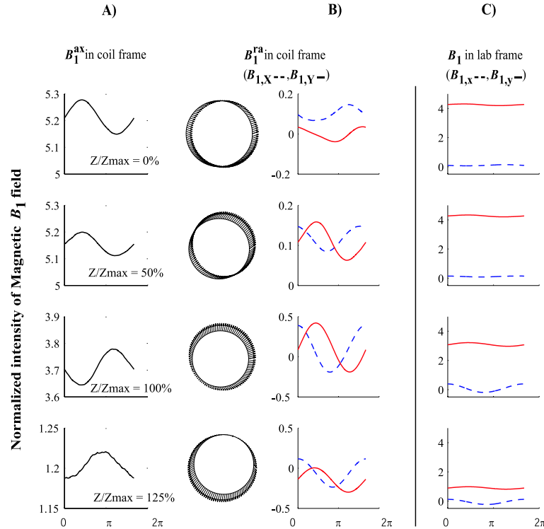
FIG. 8.6 – Set of figures equivalent to \rho = 0.5 mm : Magnetic field vectors calculated in the sample (0% and 50%) but also outside (100% and 125%). The two models can be identified at the center and at the ends of the rotor.
