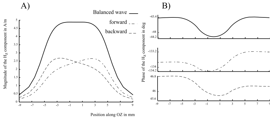
FIG. 8.7 – Result of the EM field calculation displayed at 500 MHz along the OZ axis. The magnetic field component H_z is a vector whose magnitude is presented at the left side (A). The field pattern is generated by the excitation of each port to simulate forward and backward waves and the sum of both according to the definition of balance given by Eq. 4.10. As the fields are treated as complex numbers, we have the possibility to plot the phase in degrees of these three components in (B). These curves give the phase as a function of the position along the rotor axis.
