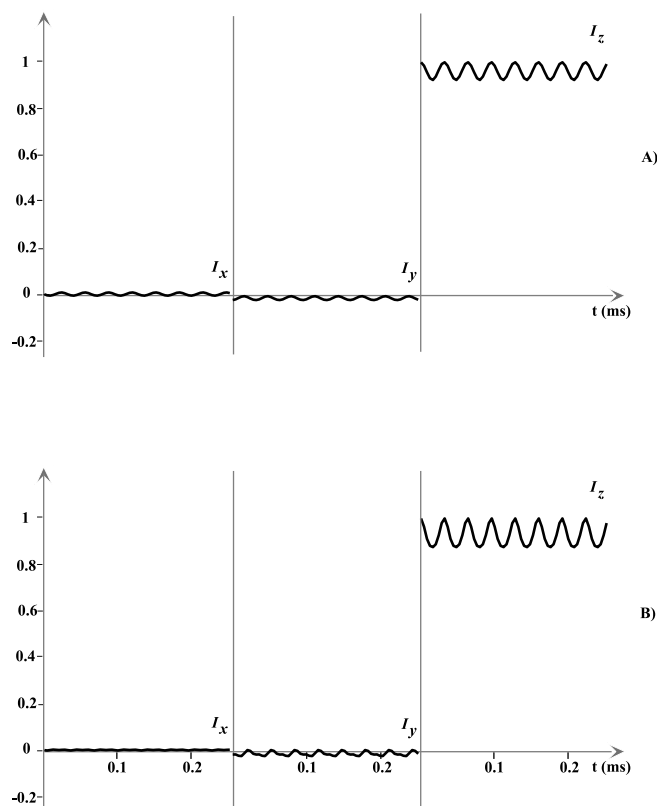
FIG. 9.2 – NMR simulations of the magnetization evolution in the Rotary Echo experiment (90^\circ)_{+x} - t - (90^\circ)_{-x} using model 1 (A) and model 2 (B). Eq.7.12 was used for model 1 and Eq.7.14 was used for model 2. The following parameters were used for the simulations : \Delta\nu = 0 , \omega_r = 2 Hz, \sqrt{2/3}\mathbf{B}_1^{ax} = 33.3 kHz, \mathbf{B}_1^{ra} = 0.1\mathbf{B}_1^{ax} , and c = 0.1 (Eq.7.15). I_x, I_y and I_z components are plotted as function of the evolution time ( t ) between the flip and flop pulses.
