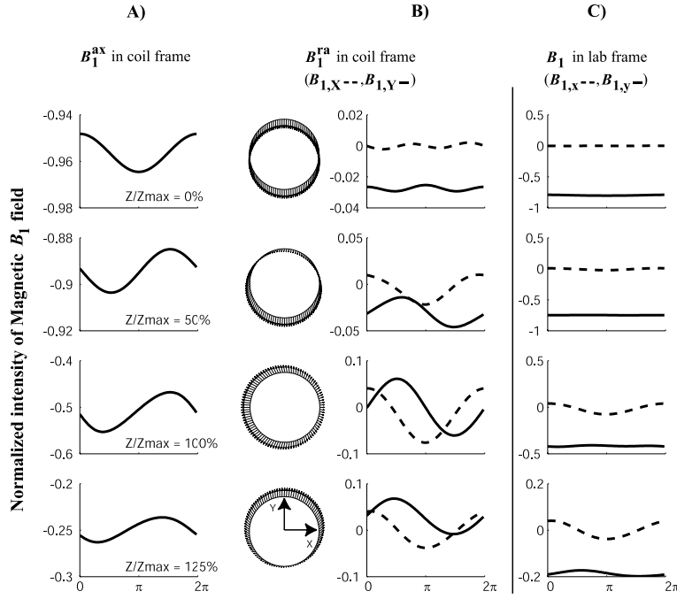
FIG. 8.2 – Set of figures \rho = 0.5 mm : Magnetic field vectors calculated in the empty coil, and displayed around circular rings of diameter 1 mm.
