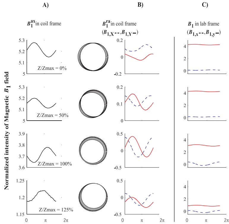
FIG. 8.6 – Set of figures equivalent to \rho = 0.5 mm : Magnetic field vectors calculated in the sample (0% and 50%) but also outside (100% and 125%). The two models can be identified at the center and at the ends of the rotor.
