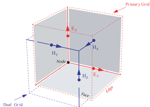
FIG. 4.1 – Dual grid known as Yee's cell.
