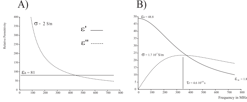
FIG. 10.3 – Models of relative dielectric permittivity, employed by CST. The left one is not suited for high frequency behaviors where dielectric decrement plays a role, and should be reserved to simpler cases. The right one encloses this one (the singularity at static frequencies is not observable) and it adds the consideration of the dispersion caused by Orientational polarization and described through the Debye model.
