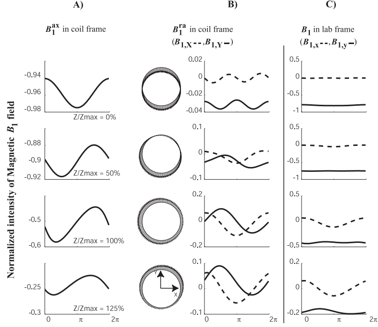
FIG. 8.3 – Set of figures \rho = 1 mm : Magnetic field vectors calculated in the empty coil, and displayed around circular rings of diameter 1.5 mm.
