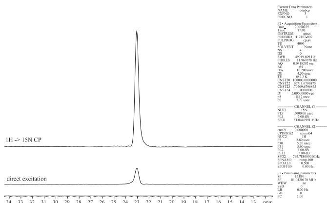
FIG. 11.12 – CP signal enhancement measurement on the ^{15}N nucleus of a ^{15}N , ^{13}C doubly labeled glycine sample packed in a CRAMPS like 4 mm rotor (31.4 mg). The ^{15}N CP as been adjusted to a 35 kHz field during the contact pulse (5 ms), for the decoupling SPINAL64 at 90 kHz was employed during 40 ms. The enhancement factor of CP as compared to direct excitation is of 7.1. Rotation speed is 11 kHz.
