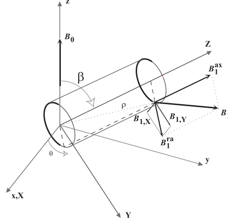
FIG. 1.5 – Representation of the (x, y, z) laboratory frame (gray) and of the (X, Y, Z) coil frame (black). The radial and axial components of the magnetic field \mathbf{B}_1 , are projected into the coil frame. Only the upper part of the rotor is displayed for clarity. As an illustration, for a given angle \theta , the spin at a distance \rho from the center, experiences a field \mathbf{B}_1 that admits as projections in the coil frame the vectors \mathbf{B}_1^{ax} and \mathbf{B}_1^{ra} .
