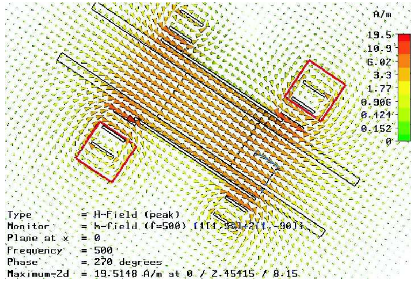
FIG. 11.3 – Axial plane cross section of the sample-loaded Z-coil for RF field simulations. The magnetic vector field distribution is indicated by small triangles. All simulations were performed with the CST Microwave Studio (CST-MWS) transient solver. Gaussian shaped pulses were applied at both terminal ports (red squares) of the coil with opposite electric phase (to simulate a balanced circuit) at 500 MHz. A 5 mm long conductive water sample was positioned in a dielectric cylinder of 18 mm length to evaluate the impact of the complex permittivity of conductive sample.
