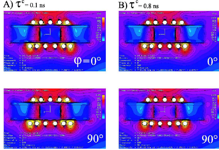
FIG. 10.5 – Distribution of the Electric field, treated as a complex field. As in the Fig. 10.4 the line correspond to a quadrature phase shift. The two columns correspond to different dielectric correlation times. Same scale was used to sort levels of electric field up to 1500 V/m. The plane selected was a OYZ passing by the coil holder, and cutting the 5.5 wires at the opposite side.
