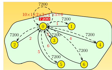
(f) MPI_Allreduce
