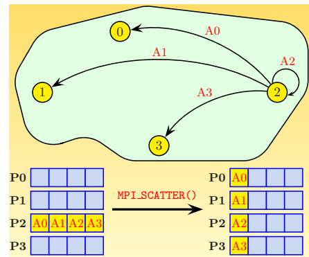
(b) MPI_Scatter
