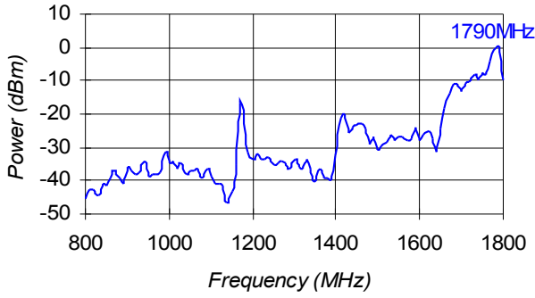
Fig. 4: Transmitted Power by the Short Aperture
