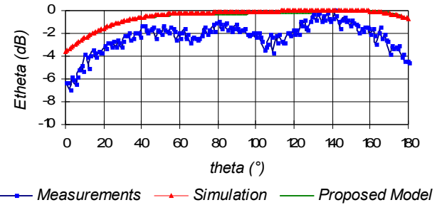
Fig. 6: Far Field Comparison for Phi=90° at f1=990 MHz
