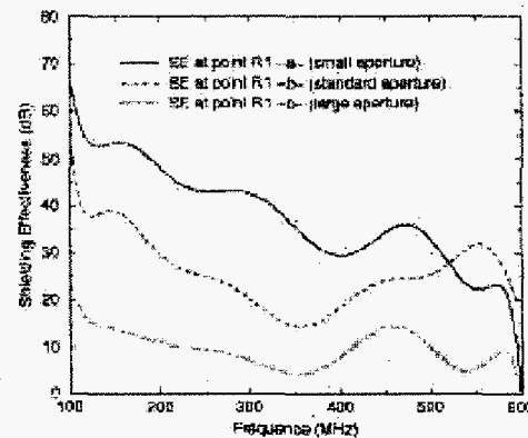
Figure 6 Shielding Effectiveness (SE) evaluated for the 3 test cases at point R1
