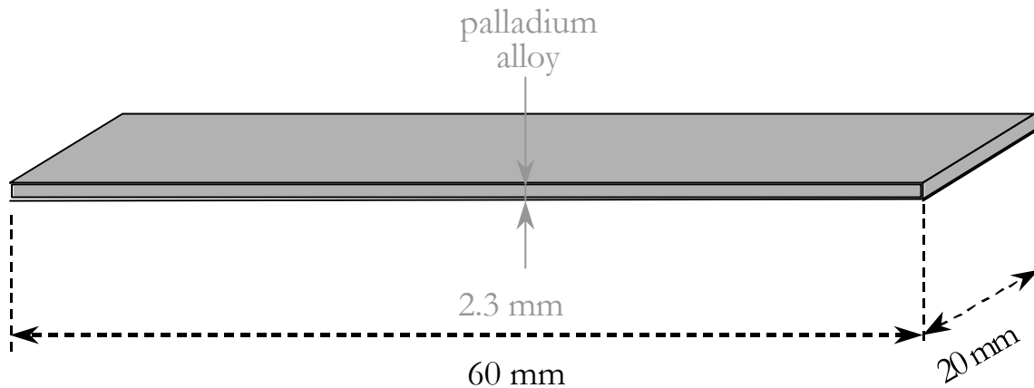
Figure 1.3: Design of analysed sample S. It represents the Pd alloy substrate before thermal processing .
