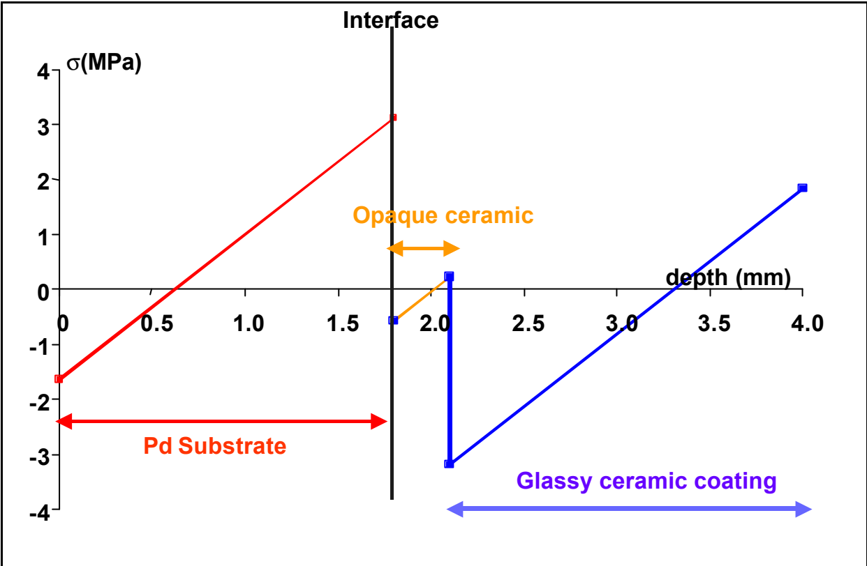
Figure 2.6: Residual stresses due to the thermal mismatch between the ceramic coating and the metal substrate.
