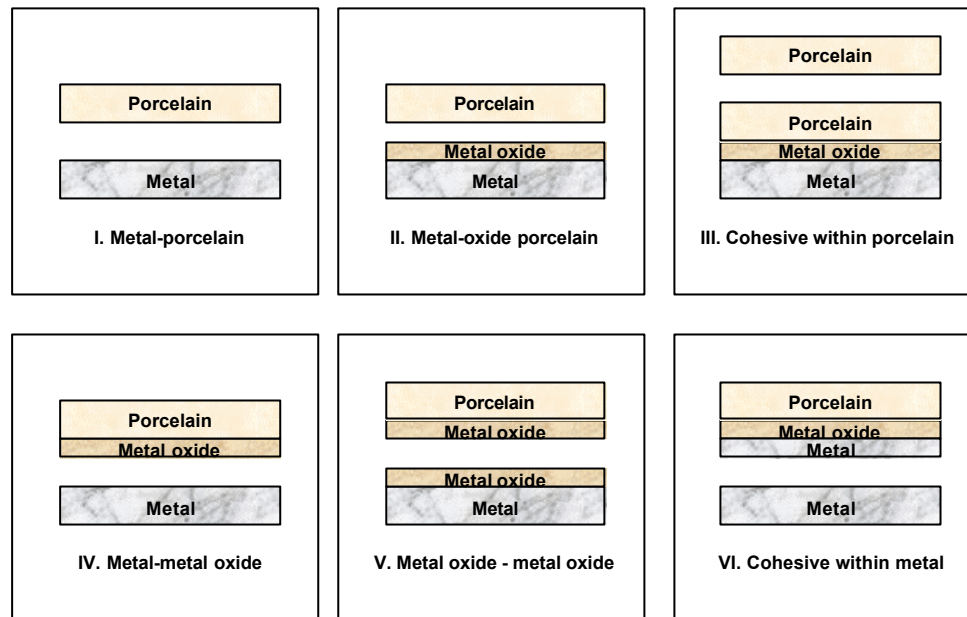
Figure 1.2: Classification of porcelain enamel failures according to the mode of failure. Type III represents cohesive failure indicative of proper bond [1.3].
