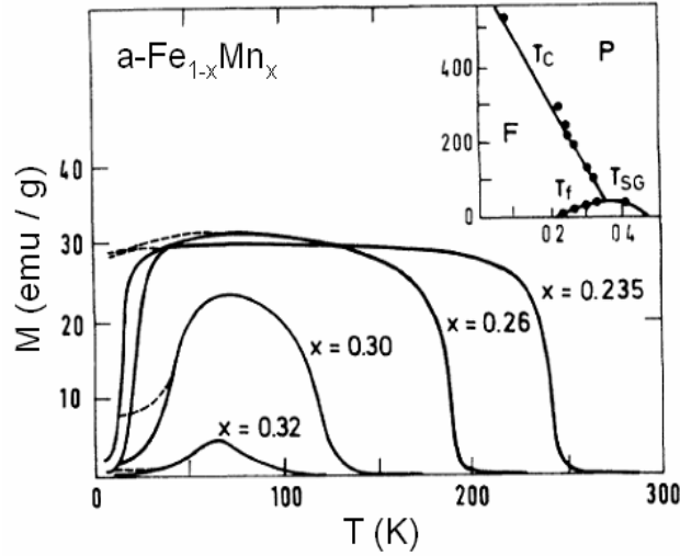
Figure 5. Low field magnetization (20 Oe) as a function of temperature for several a\text{-Fe}_{1-x}\text{Mn}_x alloys (from Ref. [Mirebeau'90]). The magnetization is measured in the zero field cooled (ZFC) and field cooled (FC) processes. In inset the corresponding typical phase diagram.
