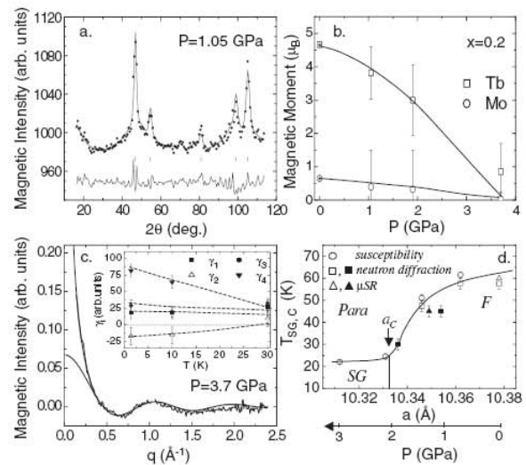
FIG. 3. (a) Magnetic intensity in x = 0.2 sample at 1.4 K and P = 1.05 GPa, with \Lambda = 4.741 Å. The solid lines show the best refinement ( R_B = 20\% ) and the difference spectrum; (b) magnetic moment versus pressure; (c) magnetic intensity of x = 0.2 at 1.4 K and P = 3.7 GPa versus scattering vector. The fit is made with the short range model (bottom line), including longer range F correlations (upper line). In the inset is the temperature dependence of the correlations coefficients; (d) phase diagram for (Tb_{1-x}La_x)_2Mo_2O_7 in the threshold region. The open symbols are measured at ambient pressure for several x contents. The solid symbols are for x = 0.2 under pressure, taking into account ESRF data to determine a(P) .
