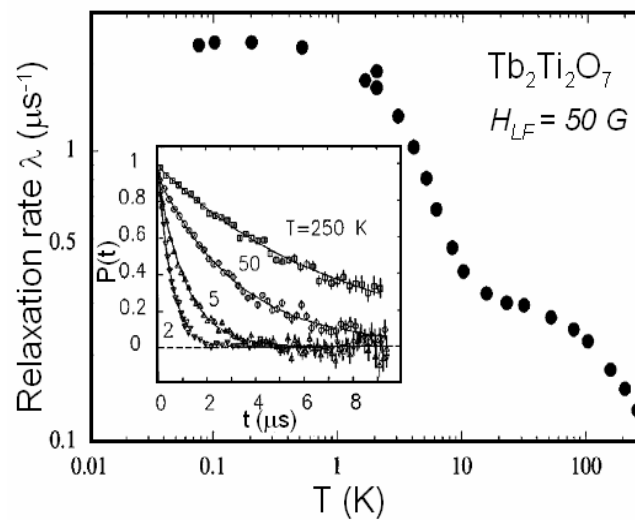
Figure 17. Tb_2Ti_2O_7 : temperature dependence of muon relaxation rate \lambda . In inset: muon spin depolarisation function P(t) for several temperatures in a small longitudinal field H_{LF}=50 G. Results are from Ref. [Gardner'99].
