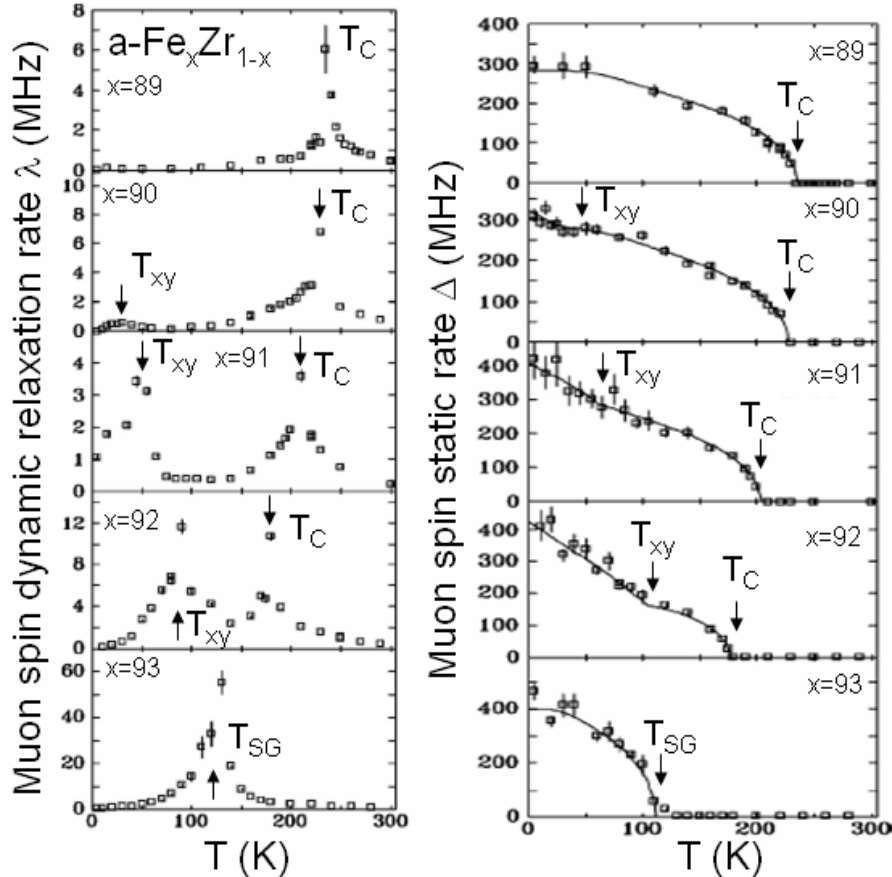
Figure 7. \mu SR for reentrant spin glasses a\text{-Fe}_x\text{Zr}_{100-x} (see Ref. [Ryan'00, Ryan'04]), for five different concentrations x=89, 90, 91, 92 and 93 : a. The muon dynamic relaxation rate \lambda against temperature; b. The temperature dependence of the static muon relaxation rate \Delta . Lines are fits to a modified Brillouin function with a linear term to include the ordering of the transverse spin components. The transition temperatures are identified as: T_C and T_{xy} , which merge for x=0.93 into T_{SG} .
