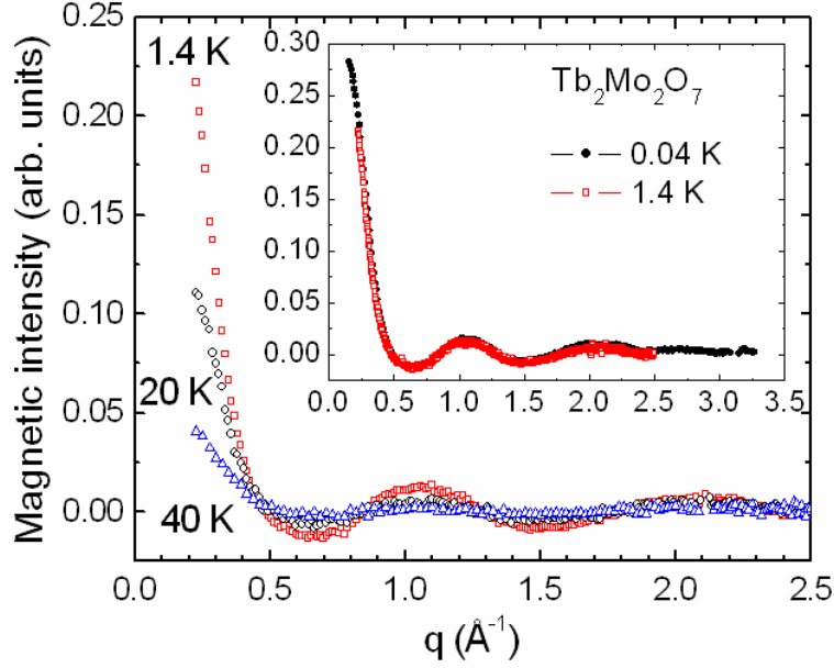
Figure 7. Magnetic intensity in Tb_2Mo_2O_7 against the scattering vector q for several temperatures: T=1.4, 20 and 40 K ( \lambda=4.741 Å) and for comparison T=0.04 K ( \lambda=2.52 Å) in the inset. A pattern at 100 K was subtracted.
