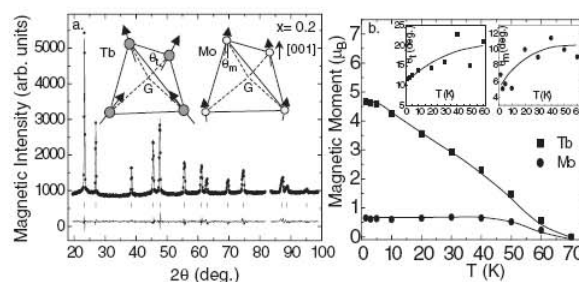
FIG. 2. (a) Magnetic intensity in the x = 0.2 sample at 1.5 K versus the scattering angle 2\theta , with \Lambda = 2.426 \text{ \AA} . A spectrum at 70 K was subtracted. The solid lines show the best refinement ( R_B = 4\% ) and the difference spectrum (bottom). In the inset is the magnetic structure of the Tb and Mo tetrahedra. (b) Ordered magnetic moments versus temperature. In the inset are the angles \theta_t and \theta_m made by Tb and Mo moments with the local anisotropy \langle 111 \rangle and the [001] axes, respectively. The solid lines are guides to the eye.
