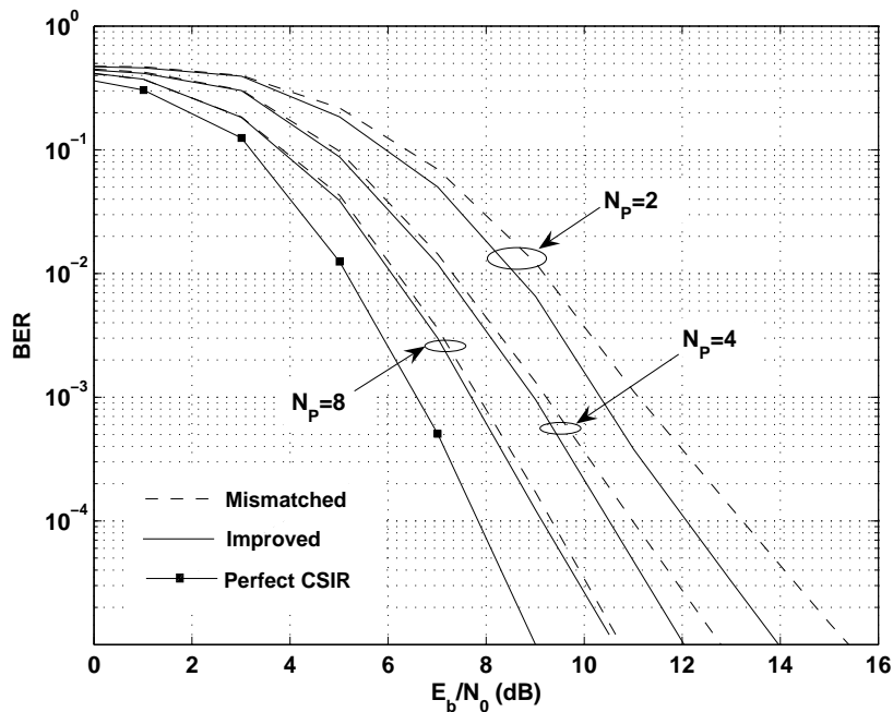
Figure 5.7: BER performance of improved and mismatched simplified turbo-PIC; (2 \times 2) MIMO with V-BLAST ST scheme, i.i.d. Rayleigh fading with N_c = 4 , QPSK modulation, training sequence length N_P \in \{2, 4, 8\} .
