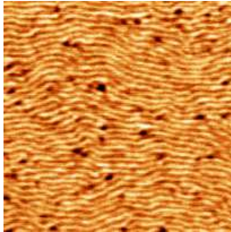
Figure III-38 : Image MFM (taille 3 \times 3 \mu\text{m} ) sur l'échantillon \text{Si}(001)/\text{Cu-Si/Fe/Pt/FePd} (35 nm)/Pd
