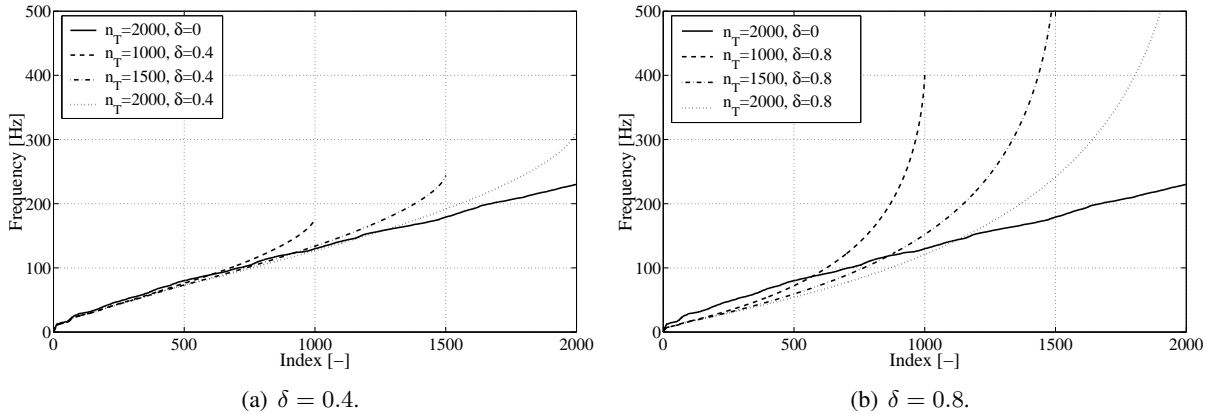
Figure 4.12: Ground-borne vibrations in the Maison du Mexique: 2000 lowest deterministic eigenfrequencies of the mean model, and mean of the random eigenfrequencies for (a) \delta=0.4 and (b) \delta=0.8 for n_T = 1000 , n_T = 1500 and n_T = 2000 .
