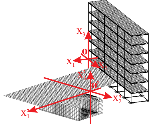
Figure 4.2: Ground-borne vibrations in the Maison du Mexique: schematic overview.
