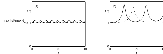
FIGURE 2.4 - \max_x|u|/\max_x\varphi_{\omega,\gamma} as a function of t for p = 4, \gamma = -1 , \delta_p = 0.001 (dashed line) and \delta_p = 0.005 (solid line). (a) \omega = 2 ; (b) \omega = 0.5 .
