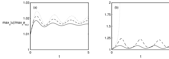
FIGURE 2.3 - \max_x|u|/\max_x\varphi_{\omega,\gamma} as a function of t for \omega = 4 , \delta_p = 0.01 , and \gamma = 1 (solid line), \gamma = 0.5 (dashed line) and \gamma = 0.1 (dots). (a) p = 3 (b) p = 5 .
