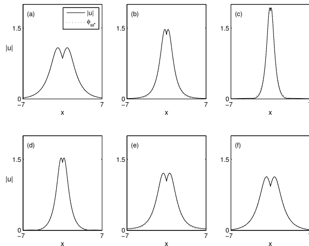
FIGURE 2.5 - |u(x,t)| (solid line) and \phi_{\omega^*(t)}(x) (dots) as a function of x for the simulation of Fig. 2.4b with \delta_p = 0.005 . (a) t = 0 ( \omega^* = 0.508 ) (b) t = 9 ( \omega^* = 1.27 ) (c) t = 10.69 ( \omega^* = 2.86 ) (d) t = 12 ( \omega^* = 1.43 ) (e) t = 15 ( \omega^* = 0.706 ) (f) t = 20 ( \omega^* = 0.58 ).
