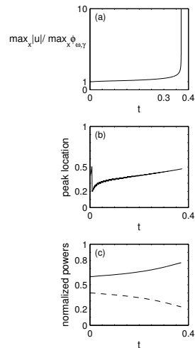
FIGURE 2.16 - (a) \max_x |u(x,t)| / \max_x \varphi_{\omega,\gamma} (b) location of \max_x |u(x,t)| and (c) The normalized powers \int_0^\infty |u|^2 dx / \int_{-\infty}^\infty |u_0|^2 dx (solid line) and \int_{-\infty}^0 |u|^2 dx / \int_{-\infty}^\infty |u_0|^2 dx (dashed line), for the solution of Fig. 2.15.
