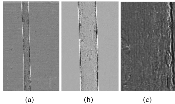
FIGURE 1. Radiographs of a 125 \mu\text{m} aluminum wire placed in the divergent x-ray beam produced by KB optics at 3 different distances z_s from the focal plane which by keeping the detector to focus distance z_d constant results in magnifications of M = \{18(a), 46(b), 278(c)\} . At the highest magnification only one edge is imaged since the field of view is smaller than the diameter of the wire.
