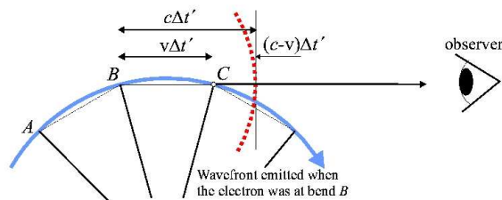
FIGURE 2. Spectral properties of the bending magnet radiation. A stationary observer only receives the radiation as it traverses an arc between points B and C.
