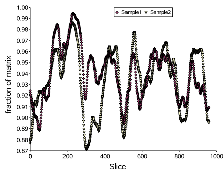
FIGURE 18. The volume fraction of the matrix relative to the total volume for the initial material - S1 (violet diamonds) and for the 12 h annealed sample - S2 (yellow triangles). The slice per slice variation of Al_2Cu particles after annealing follows closely the initial distribution and the mean values are very similar if the whole volume is considered.
