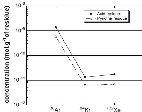
Fig. 2. Orgueil acid and pyridine-swollen residue concentration of heavy noble gases. Our results for Ar, Kr and Xe concentrations in Orgueil acid residue are close to those reported in the literature [10,35] and due to the log-scale representation no significant difference could be observed. In order to increase the readability of the figure, we do not represent data from literature. Errors are typically include in the 0.5–3% range. As results for both pyridine residues are very similar, we plot only the residue treated with pyridine for 1 h.
