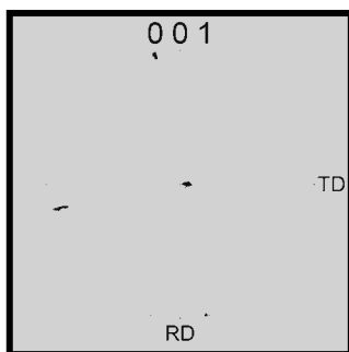
Figure II.d - Figure de pôles (001)
