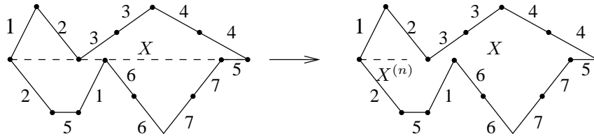
FIGURE 10. The transformation T is a first return map of the vertical flow on a union of saddle connections.
