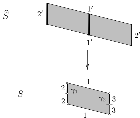
FIGURE 1. An unfolded flat surface S with two \hat{h} omologous saddle connections \gamma_1 and \gamma_2 .
