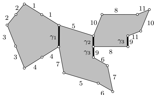
FIGURE 2. Unfolded flat surface with three \hat{h} omologous saddle connections \gamma_1, \gamma_2 , and \gamma_3 .
