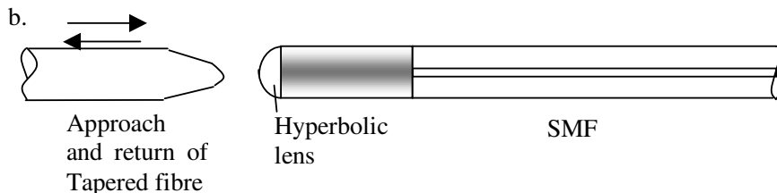
Figure 1 : Principle and fabrication process of the microlensed GI fibre
