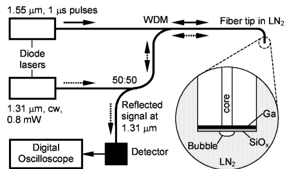
FIG. 1. Schematic of the diode-laser/fiber-optic arrangement for generation and optical study of bubbles in liquid nitrogen, with enlarged detail of the fiber tip.
