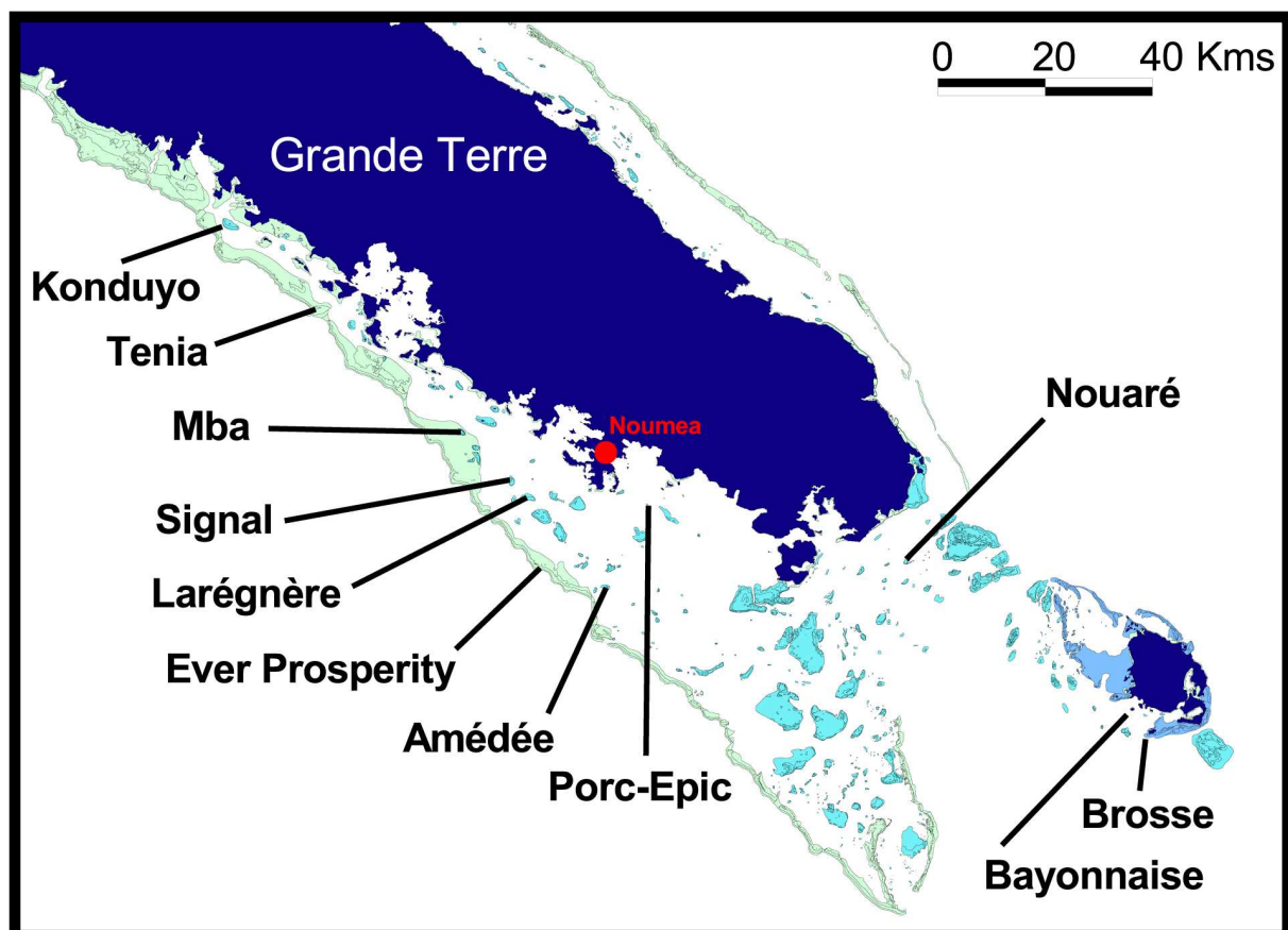
FIG. 4 – The South-West Lagoon of New-Caledonia. Dark-blue areas represent the emerged land (Main land and islets) ; light-blue areas, the reef flats and light-green areas the barrier-reef and the fringing reefs.
