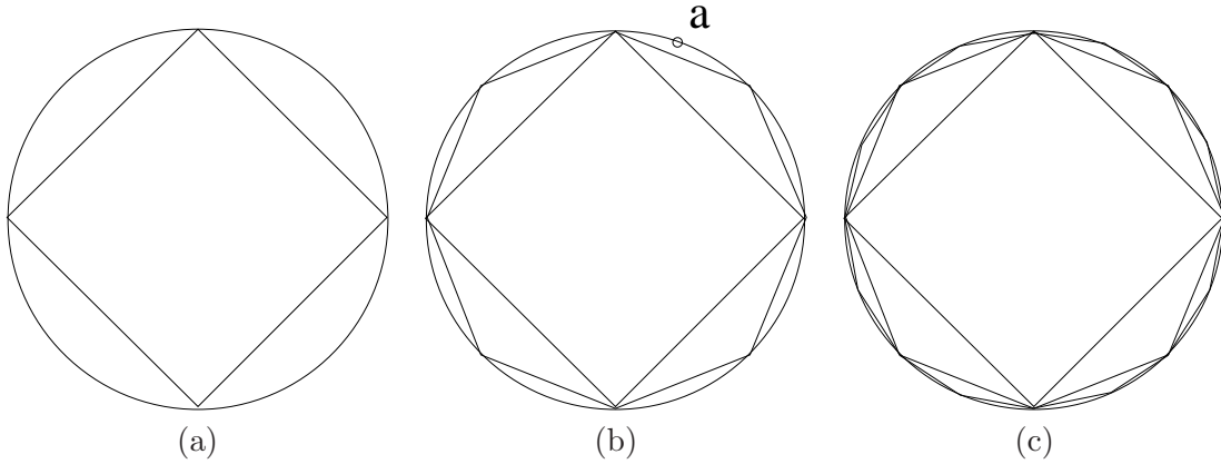
Figure 2.1: (a) Symmetric semi-definite positive matrix with trace equal to 1 and cone of diagonal dominant matrix. (b) Cone \mathcal{C}(\mathcal{S}_1) , a is on the border of the semi-definite positive matrix. (c) Cone \mathcal{C}(\mathcal{S}_2) .
