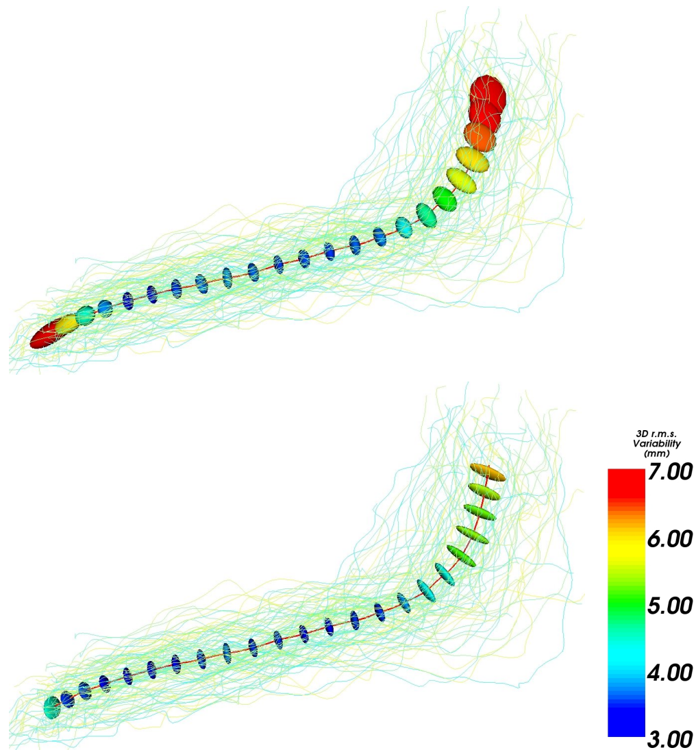
Figure 12.1: Canceling the tangential component. Top: Covariance matrices extracted along the mean Sylvian Fissure as in section 11. Bottom: The same tensors after canceling the tangential component. A small tangential value is kept for visualization purposes (tensors should be flat).
