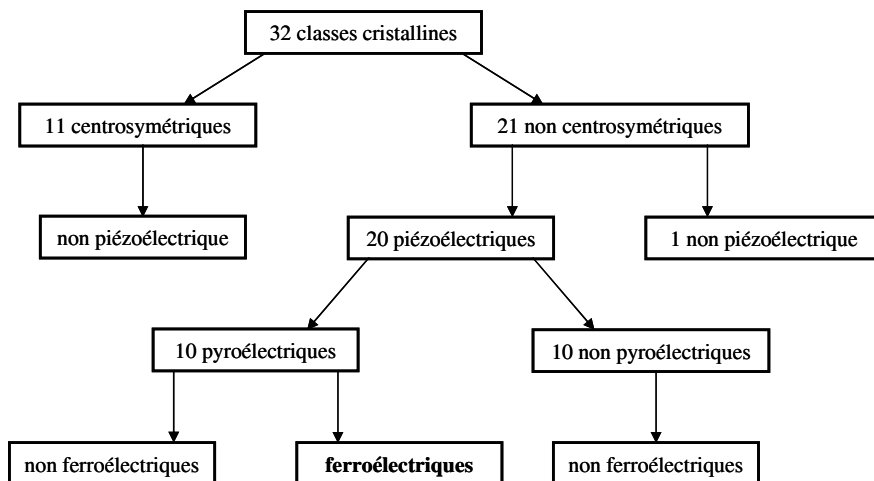
Fig. II.1. Classes cristallines.
