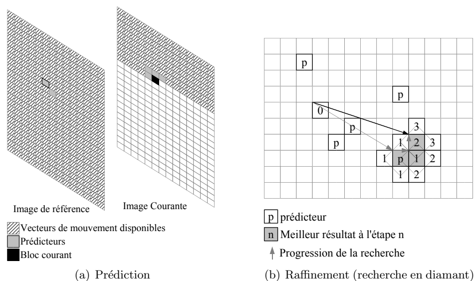
FIG. 2.8 – Algorithme EPZS
