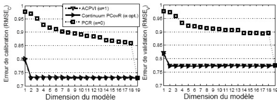
(b) Principal covariate regression
