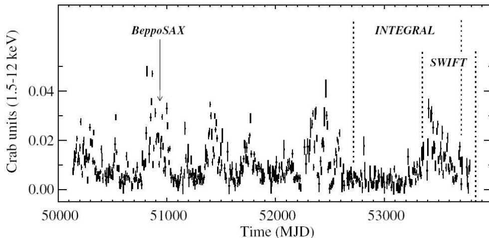
Figure 7.1: The 4U 1954+319 RXTE /ASM light curve in the 1.5–12 keV energy band (data-averaged over a 7-day interval). The ASM count rate were converted to flux using 1 \text{ Crab} \approx 75 \text{ cts/s} 168 .
