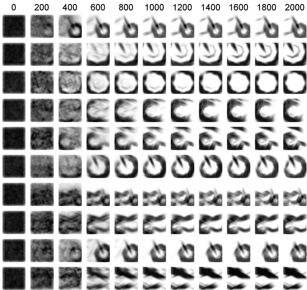
Figure 2.4: Evolution of reconstructions for motorbike features.
