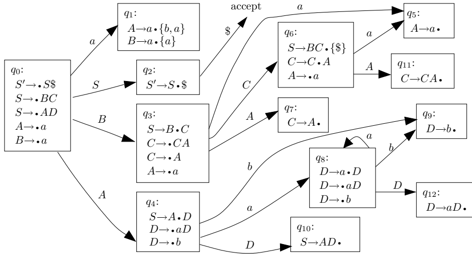
Figure 5.1: The LALR(1) automaton for \mathcal{G}_{12} .
