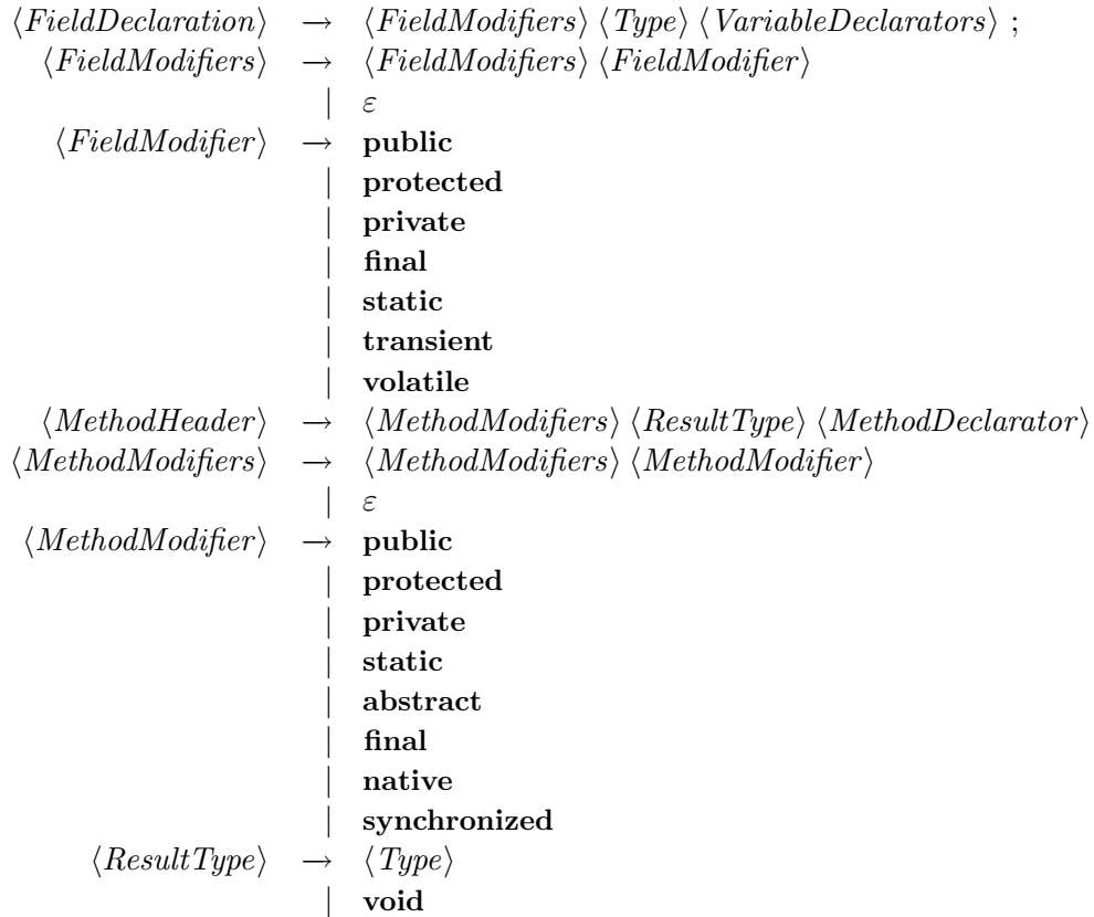
Figure 3.1: Fields and methods declarations in Java. \langle FieldDeclaration \rangle and \langle MethodHeader \rangle appear in the same context, and both \langle VariableDeclarators \rangle and \langle MethodDeclarator \rangle first derive identifiers.
