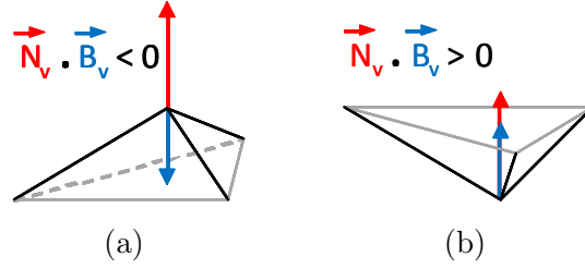
Figure 5.6: Description of the roughness measure at a given vertex v . (a) In case of a local convexity, the outer normal (red) and barycentric normal (blue) have a negative dot product. (b) In case of a local concavity, the dot product is positive.
