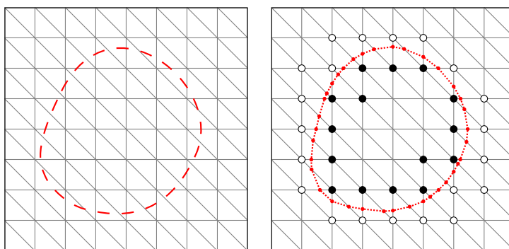
Figure 2.17: Simplicial decomposition and corresponding approximation of a contour. The control points of the snake (in red) evolve on the simplicial grid.
