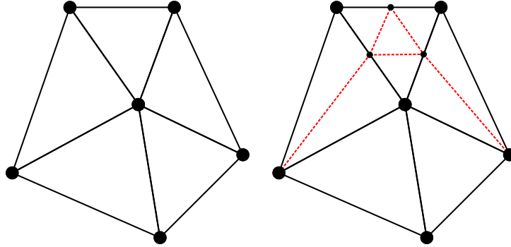
Figure 2.11: Re-sampling schemes in the GDM framework. The re-sampled face is replaced by four new faces, and neighbor faces are adjusted to respect the triangular topology.
