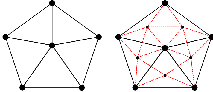
Figure 2.14: \delta -snake global refinement scheme. A new vertex is created in the barycenter of each old face, and is connected to the three vertices of the old face as well as the new vertices created in the neighbor faces.
