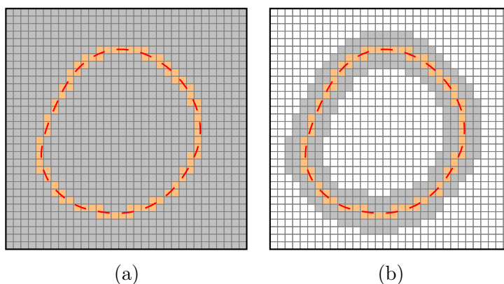
Figure 2.23: Principle of the Narrow-band optimization. In the original level set method (a), \varphi is updated over the whole image domain (gray pixels). In the narrow-band method (b), \varphi is updated only within a band located around \tilde{\varphi} , yielding a lower complexity. If \tilde{\varphi} hits the edge of this narrow band, a new narrow band of same width is computed.
