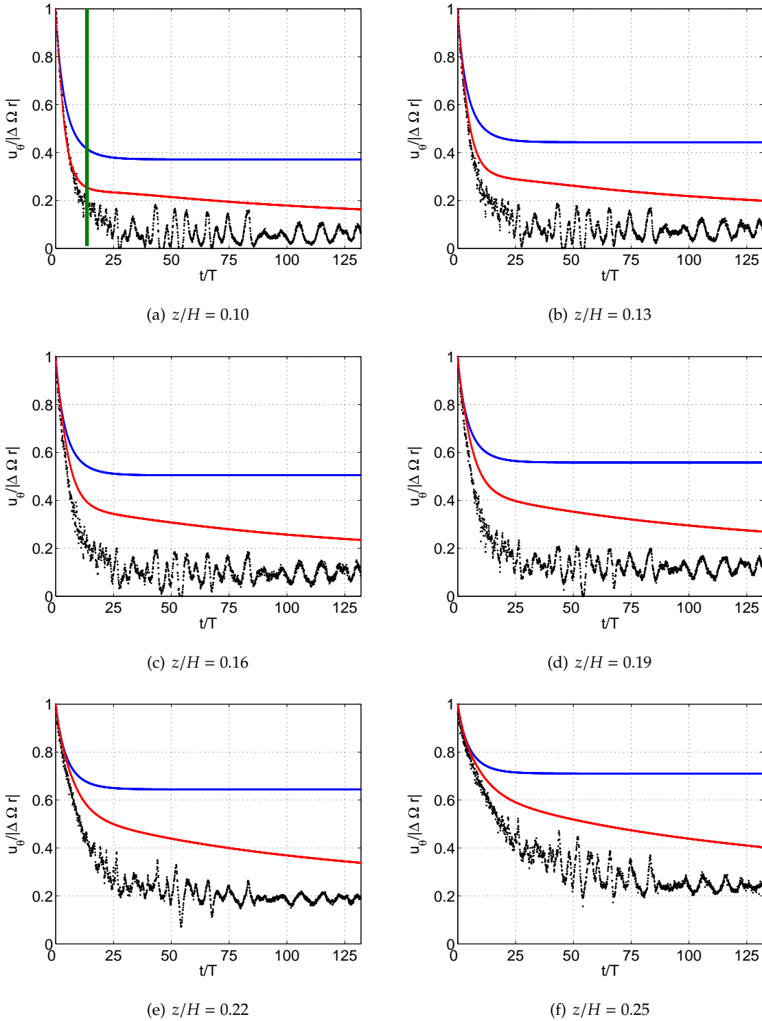
Fig. 6.8: SIDE VIEW UP 3 ( (\epsilon, Bu) = (0.32, 4.34) ) - non-dimensional azimuthal velocity [-] - temporal evolution at different vertical locations: —●— experimental results; —●— Walin's theory; —●— our model. The spin-up time has been reported in fig. 6.8(a) as a green vertical line.
