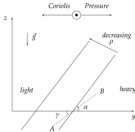
Fig. 2.3: The slope of the isopycnal surfaces with respect to the horizontal.
