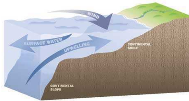
Fig. 1.1: Where Ekman transport (§ 3.1.2) moves surface waters away from the coast, these are replaced by denser water that wells up from below in the process known as coastal upwelling . Note that the continental shelf is the extended perimeter of each continent. The shelf usually ends at a point of increasing slope, named shelf break . The sea floor below the break is the continental slope .
