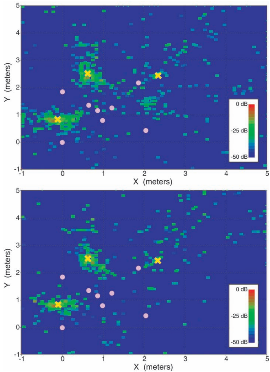
Figure 6.7 Energy localization map for a 28s.-long audio sequence featuring 3 speakers inside a room (indicated by the three yellow crosses). Light-purple dots show the location of the 8 microphones. The top map is computed using AMDF-based TDOA estimation while the bottom map is computed using GCC-PHAT. Both maps were computed using 8 subbands and corresponding energy is integrated over the entire duration of the sequence.
