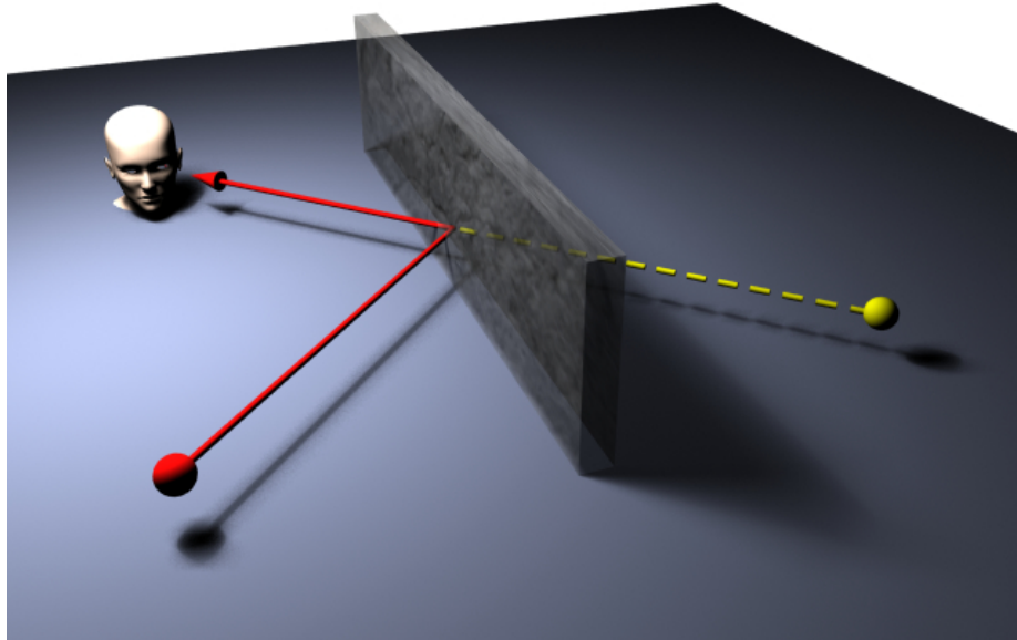
Figure 3.4 The reflection of the sound source (red sphere) solved with a source-image technique. A virtual source (yellow sphere) is created reducing the problem to that of a direct sound source.
