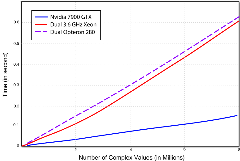
Figure 4.7 Comparison of 1D Fast Fourier Transform on CPU and GPU [Govindaraju et al., 2006].
