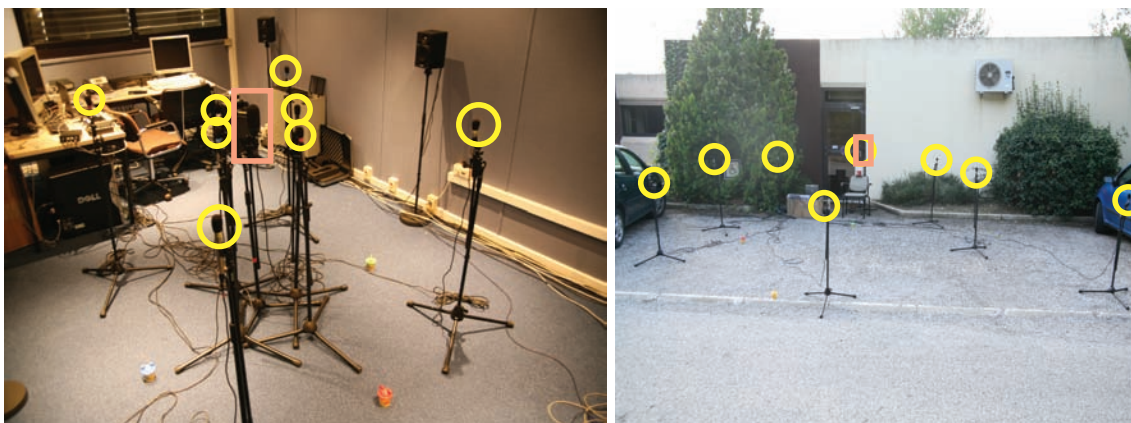
Figure 7.4 Example recording setups. We used 8 omnidirectional microphones (circled in yellow) to capture the auditory scene as well as a Soundfield microphone (highlighted with a light red square) to simultaneously record a B-format version. A binaural recording using microphones placed in the ears of a subject provided a reference recording in each test case.
