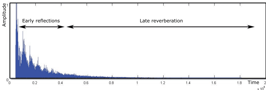
Figure 3.3 Example of room impulse response composed of the direct sound, early reflections and late reverberation.
