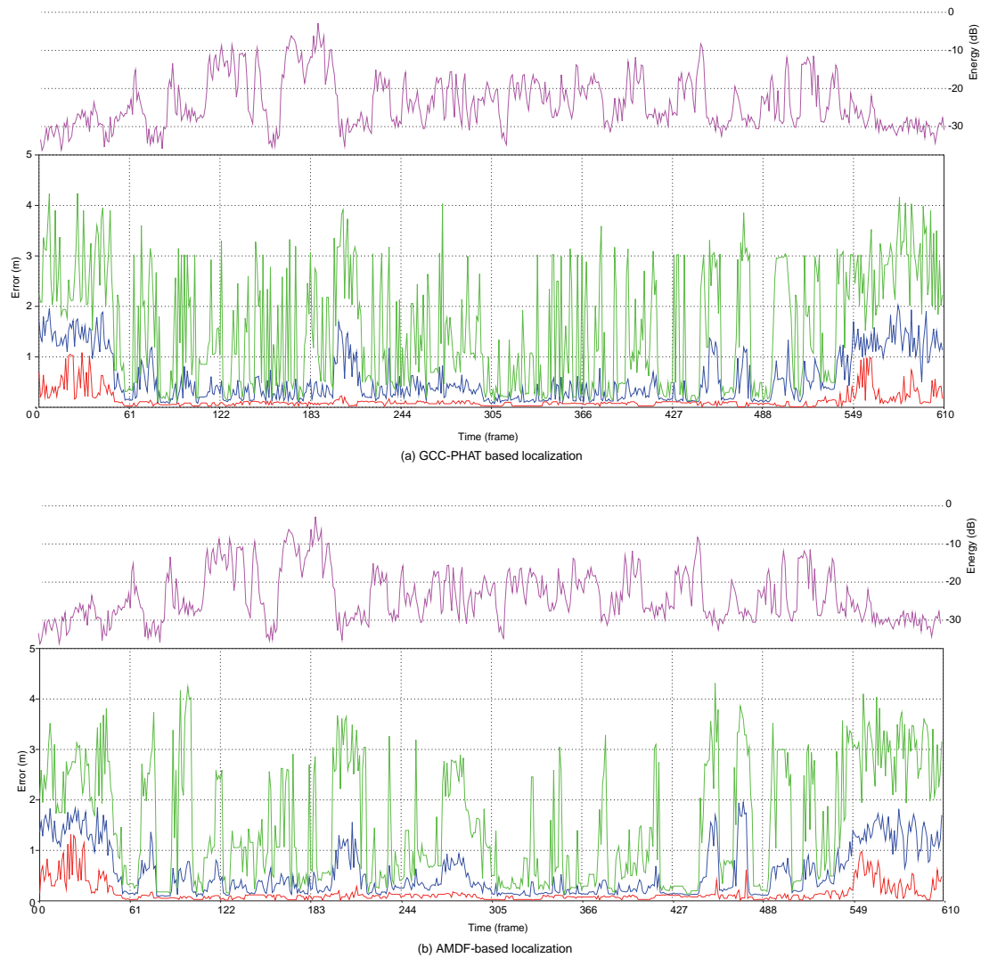
Figure 6.10 Localization error for the same audio sequence as in Figure 6.7. computed over 8 subbands. Averaged error over all subbands is displayed in blue, maximum error in green and minimum error in red. The top (magenta) curve represents the energy for one of the input recordings and shows its correlation with the localization error (clearly larger when the energy drops out).
