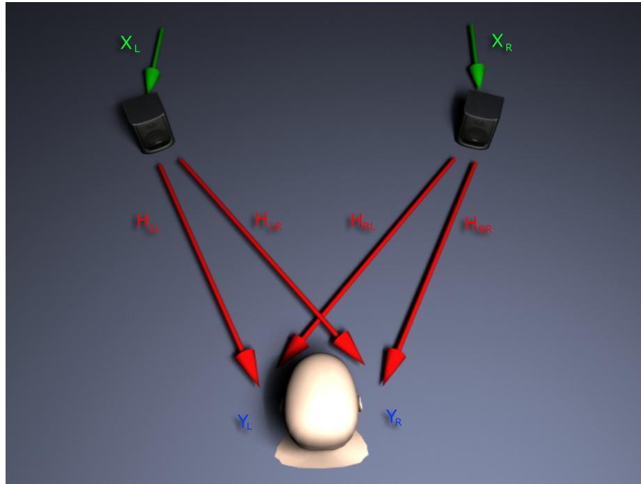
Figure 3.8 Transaural technique overview. the perceived signal Y_r, Y_l is a mixture of the signal X_l and X_r convolved by a filter H .
