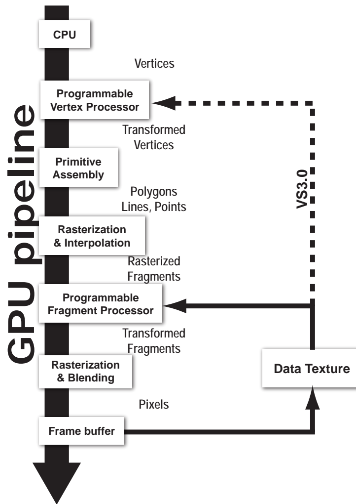
Figure 4.1 GPU pipeline. The vertex processor and the fragment processor are totally programmable.
