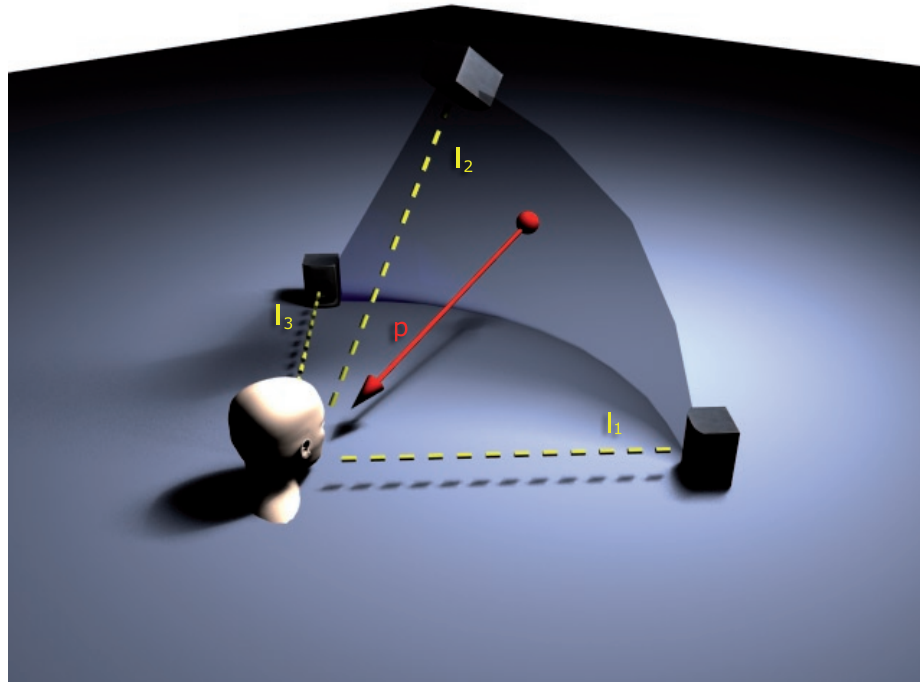
Figure 3.7 Vector Base Amplitude Panning. A phantom source (red sphere) is created using N speakers ( N=3 in this example).
