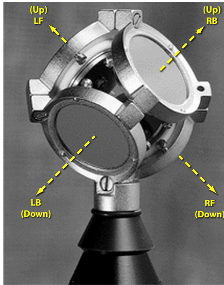
Figure 3.9 Four-capsule microphone positioned in a tetrahedron. The soundfield can be defined by an omnidirectional pressure and three difference pressures in X, Y, Z direction(©Soundfield).
