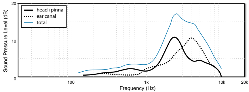
Figure 2.2 Transfer function of the outer ear from a sound at 45 degrees in the horizontal plane, related to the head and pinna and to the ear canal. This figure also show the combined result which emphasizes the frequency range of speech.
