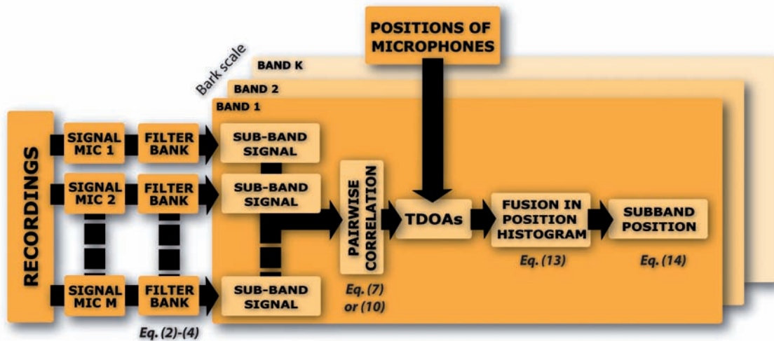
Figure 6.3 Overview of the analysis algorithm used to construct a spatial mapping for the acquired soundscapes.
