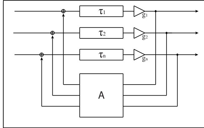
Figure 3.5 Feedback delay networks topology. A is the feedback matrix, \tau_i are the delays and g_i are the gains.
