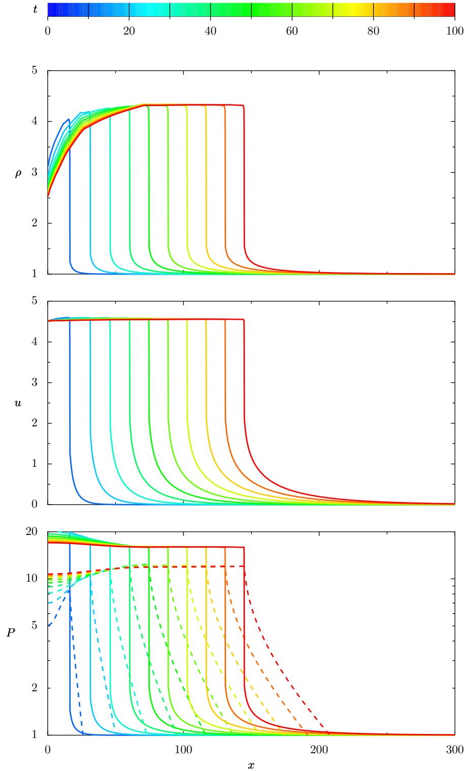
Figure 5.4: Time evolution of the hydrodynamical profiles for a modified shock (with D(p) \propto p and p_{\max} = 10 ).
