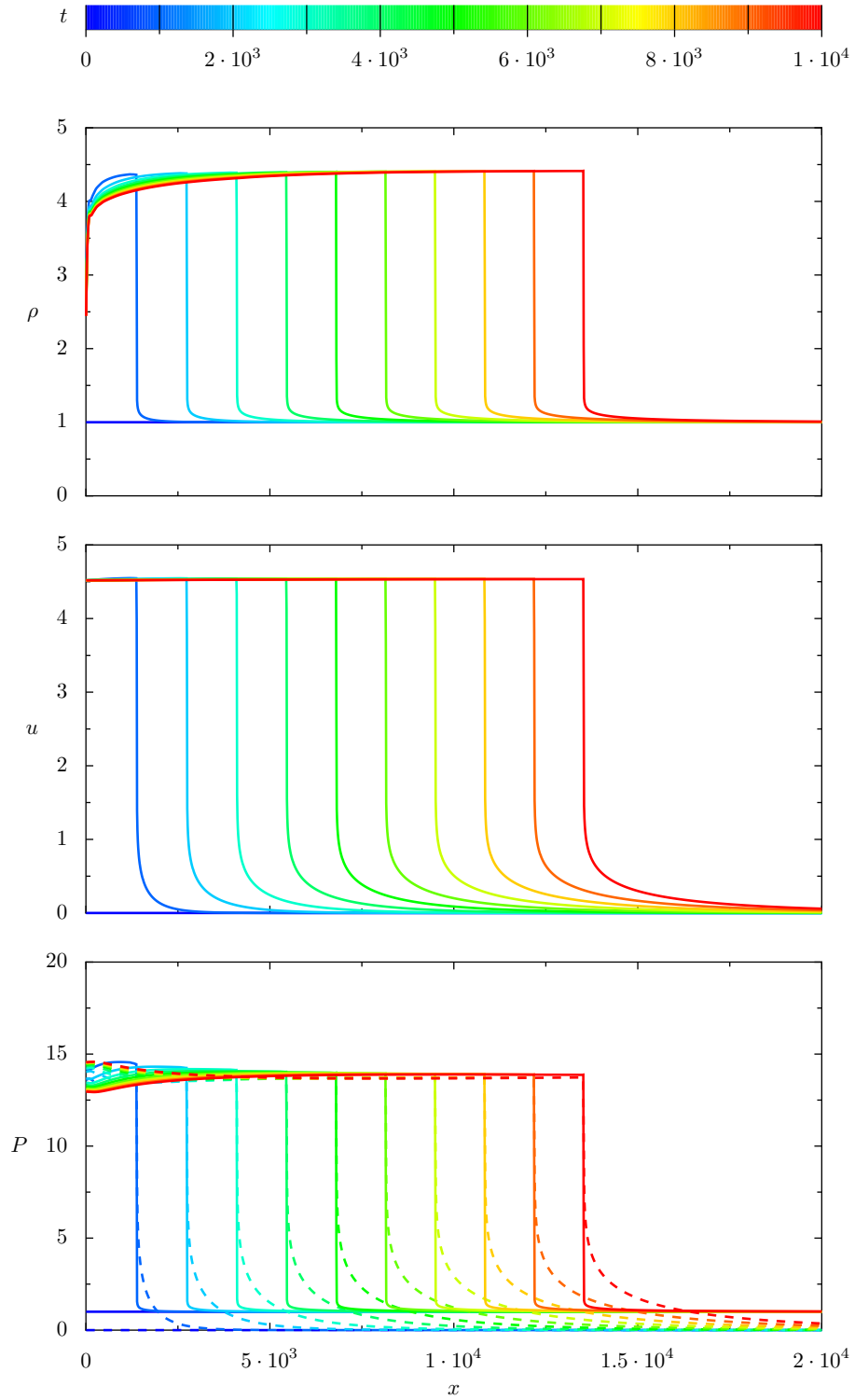
Figure 5.9: Time evolution of the hydrodynamical profiles for a modified shock (with D(p) \propto p and p_{\text{max}} = 10^3 ).
