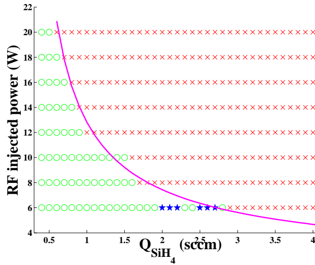
Figure III.17: Aggregation instability appearance areas in a P_{rf}/Q_{SiH_4} plane. Instability: \circ , no instability: \times , particular case: \star
