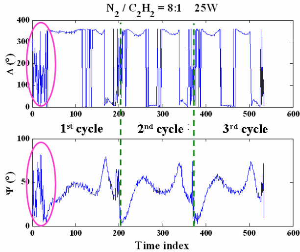
Figure V.13: Typical ellipsometric spectra: time evolution of \Delta and \Psi .
