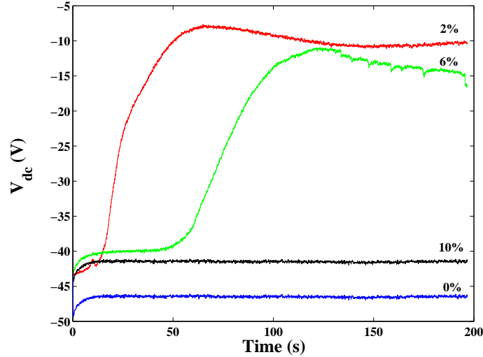
Figure V.6: Time evolution of V_{dc} for different dilutions.
