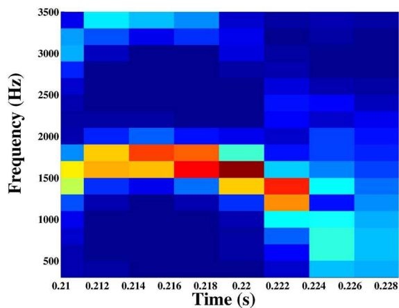
FIG. 3. (Color online) Time evolution of the frequency of the instability.
