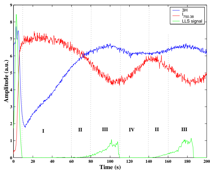
Figure IV.3: Time-evolution of 3H, I_{A_{7^*}} and LLS during dust particle successive generations in an Argon-Silane plasma.
