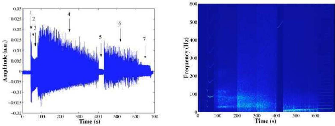
(a) Time evolution of the amplitude of the discharge (b) Spectrogram of electrical measurements corresponding to (a) and describing the frequency evolution during dust particle growth (ac component). Instabilities appear around of DPGI as a function of time. 40 s after plasma ignition. Successive phases are numbered from 1 to 7.
