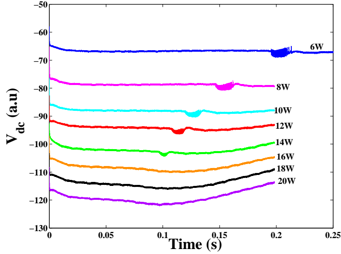
Figure III.8: Time-evolution of the self-bias voltage versus the injected power for Q_{SiH_4} = 0.8 scm.
