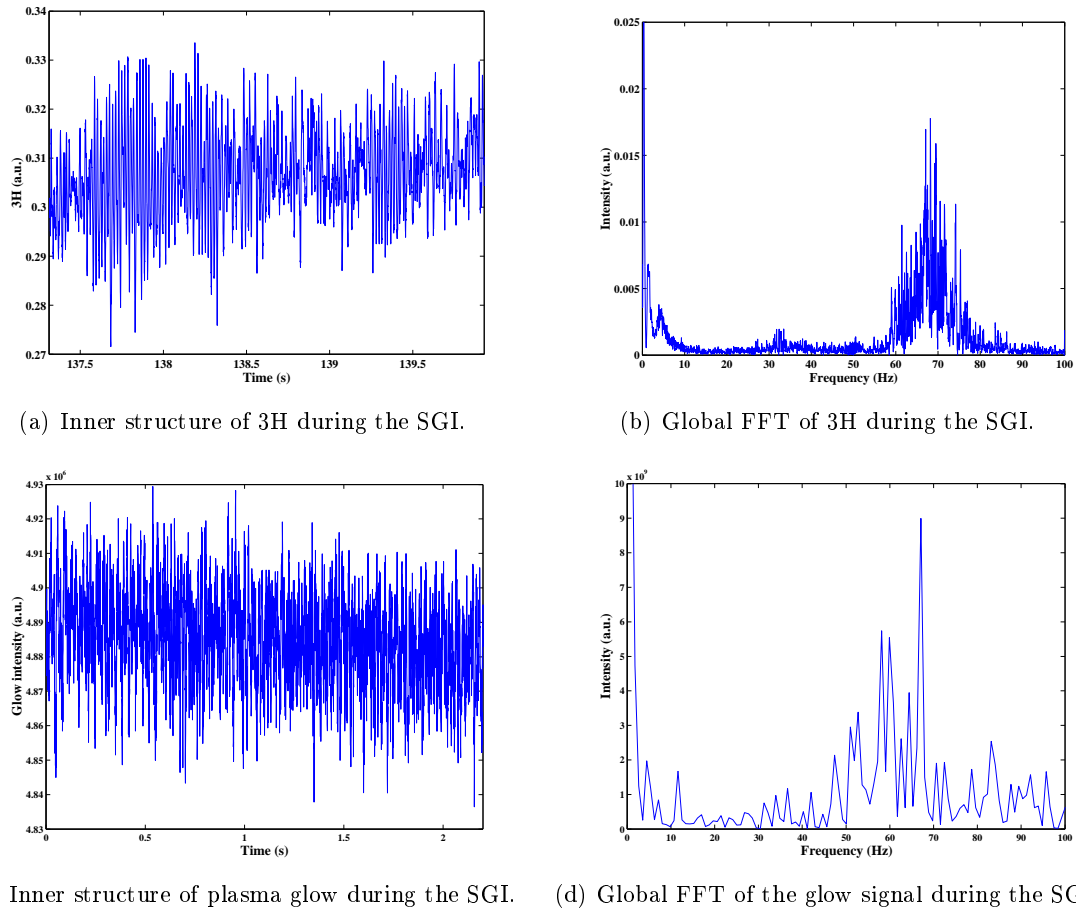
Figure IV.9: Time-evolution of 3H and plasma glow with their corresponding FFT during the SGI.
