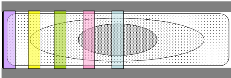
Figure IV.6: Model of the void region in the Ar/SiH 4 discharge.
