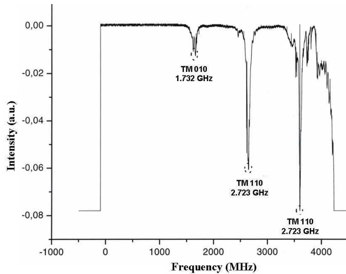
Figure II.12: Cavity spectrum.
