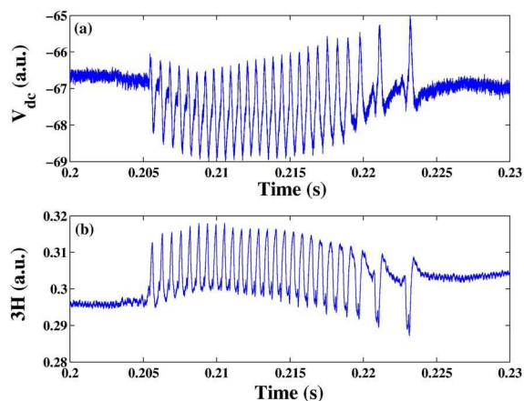
FIG. 2. (Color online) Time evolution of the instability (a) on the self-bias voltage and (b) on the third harmonics of the discharge current.
