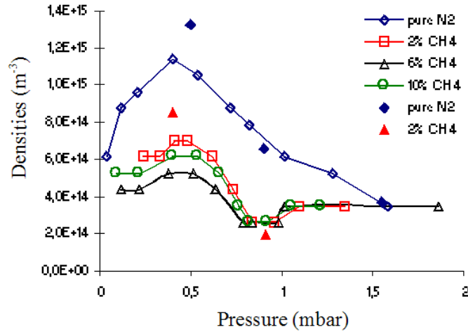
Figure V.9: Evolution the electron (empty symbols, microwave resonant cavity measurements) and ion (full symbols, Langmuir probe) densities as a function of pressure both in N 2 and N 2 /CH 4 plasmas.
