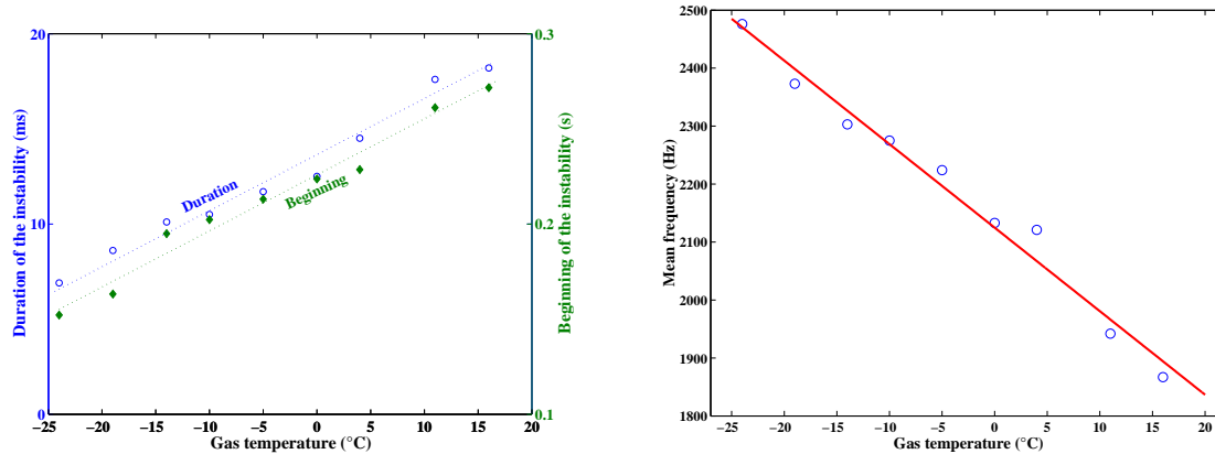
(a) Beginning and duration of the instability as a function of low gas temperature (b) Mean frequency as a function of low gas temperature
