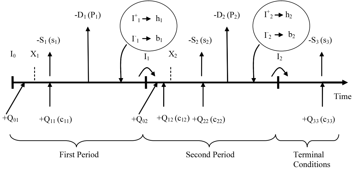
Figure 4.1: Decision process
