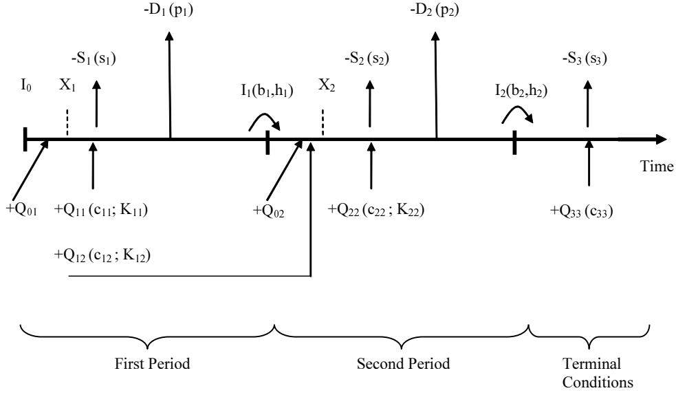
Figure 5.1: Decision process
