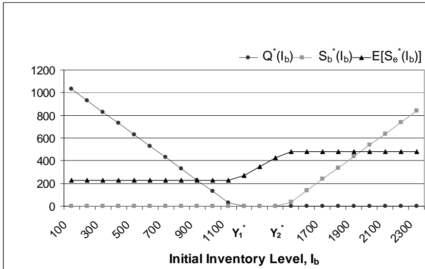
Figure 3.4: Optimal policy
