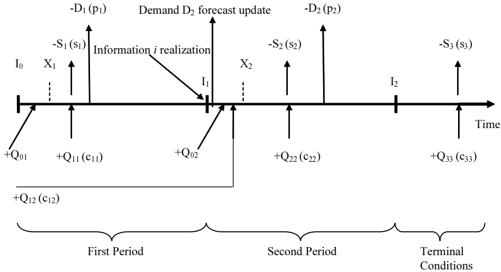
Figure 6.1: Decision process
