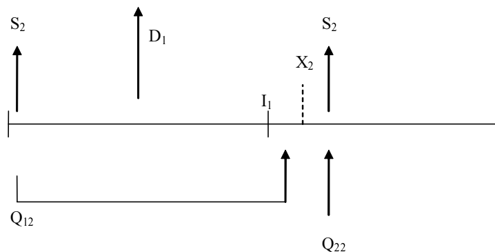
Figure 4.3: Decision process
