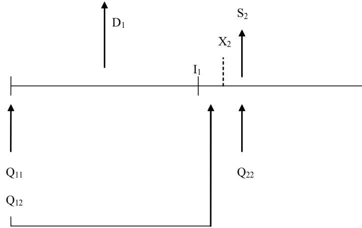
Figure 4.2: Decision process
