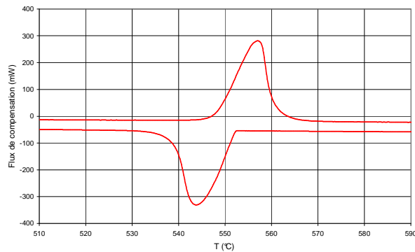
(a) LiBr
