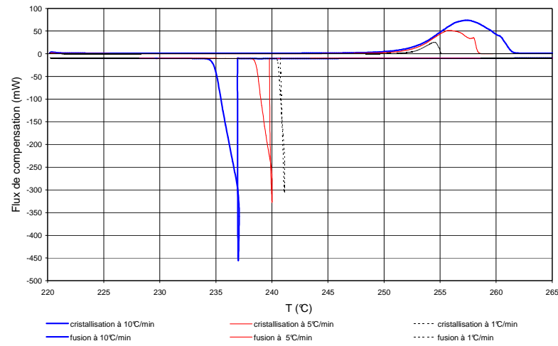
(a) \text{LiNO}_3
