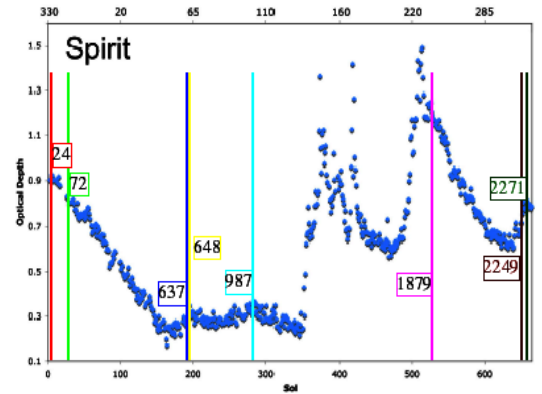
Fig. 2.1. Opacité atmosphérique (cf. page 25 ) [Bell et al., 2006a], [Lemmon and Athena Science Team, 2006]
