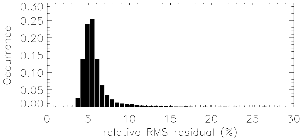
Fig. 4.16. Histogram of the relative score (rms residuals) given in %; one notes a gaussian distribution centered on 5% with a residual tail beyond 8%.
