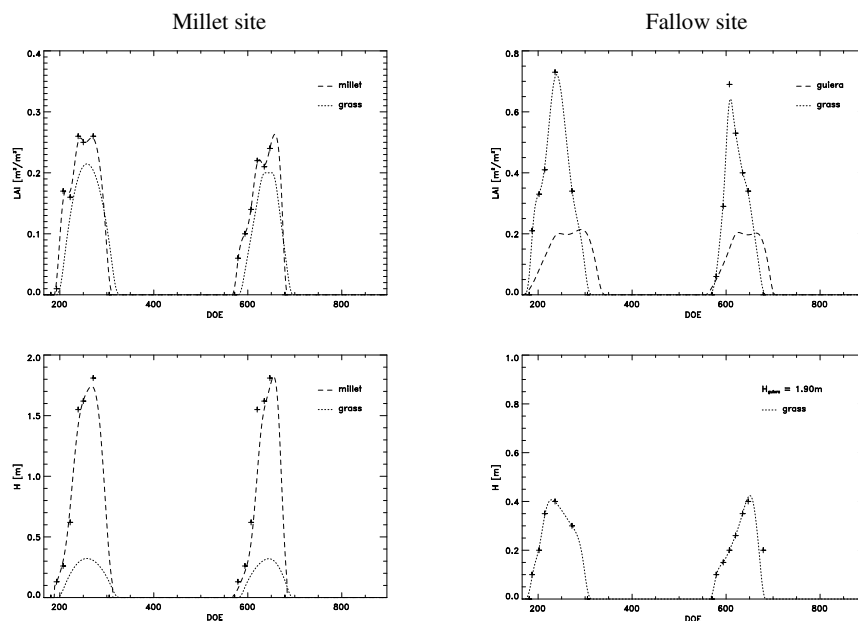
Figure 2 Vegetation parameters (LAI, h) seasonal evolution for the two experimental sites : millet and fallow
