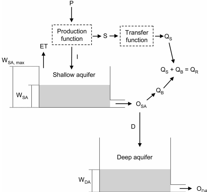
Figure 3-10 Structure of the conceptual lumped model built specifically to the F  f   catchment.
