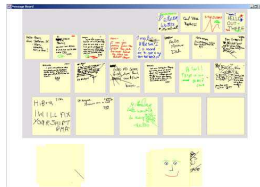
Figure 1. messageProbe
