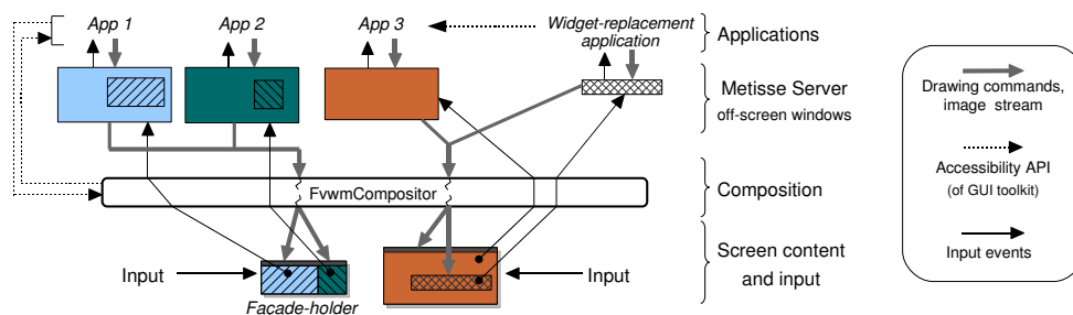
Figure 4: Illustration of input event and image flow in Façades system
