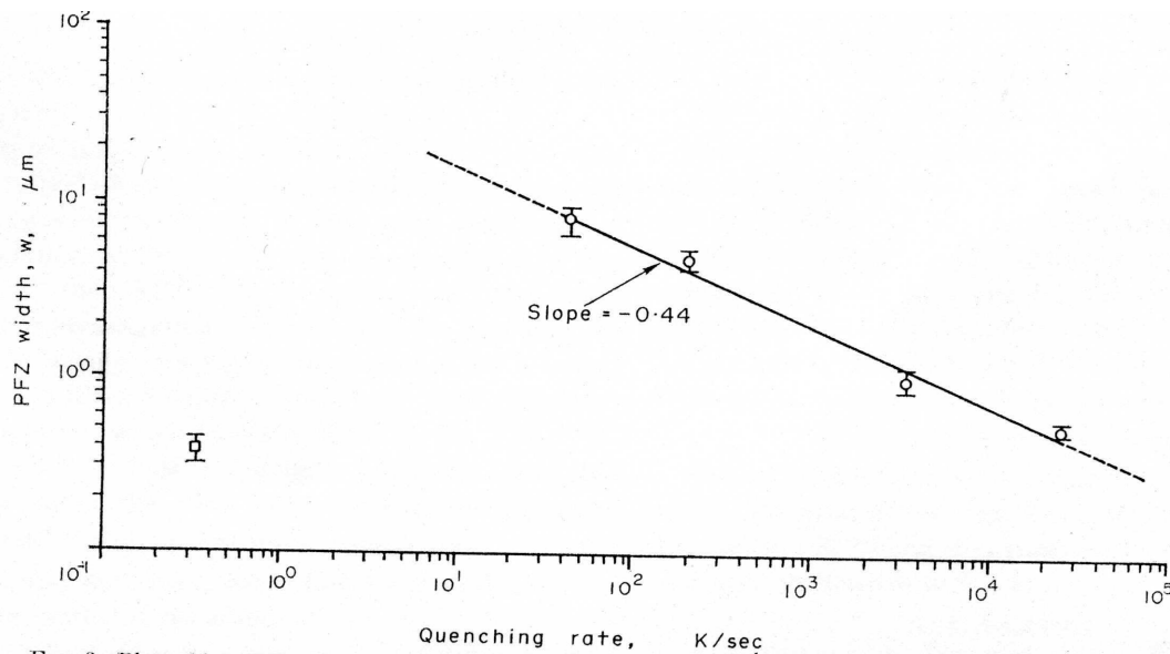
FIG. 3. Plot of log (PFZ width) vs log (initial quenching rate). The slope is -0.44 which compares with the predicted value of -0.50 .
