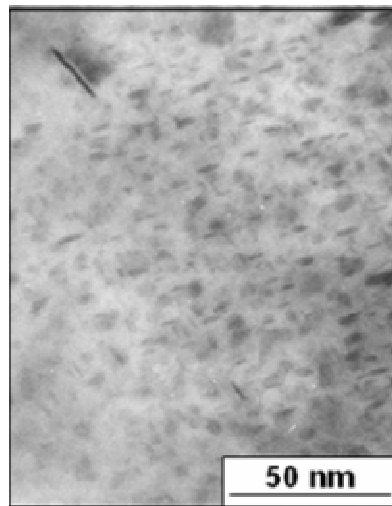
Figure III.27.b : 7449 T651
