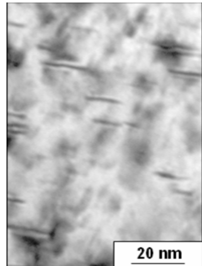
Figure III.27.e : PA T7651
