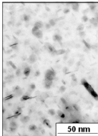
Figure III.27.d : 7449 T7651
