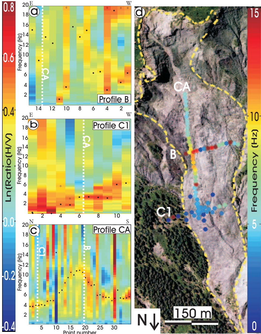
FIG. 7.5 – (a) ratio of the vertical and horizontal component (H/V) of seismic noise analysis and seismic noise network results obtained at the Super-Sauze mudslide along the profile B, (b) the profile C and (c) the longitudinal profile CA. (d) the picked frequency is displayed in colour, including H/V measurements acquired during the seismic noise network experiment. See text for more explanations.
