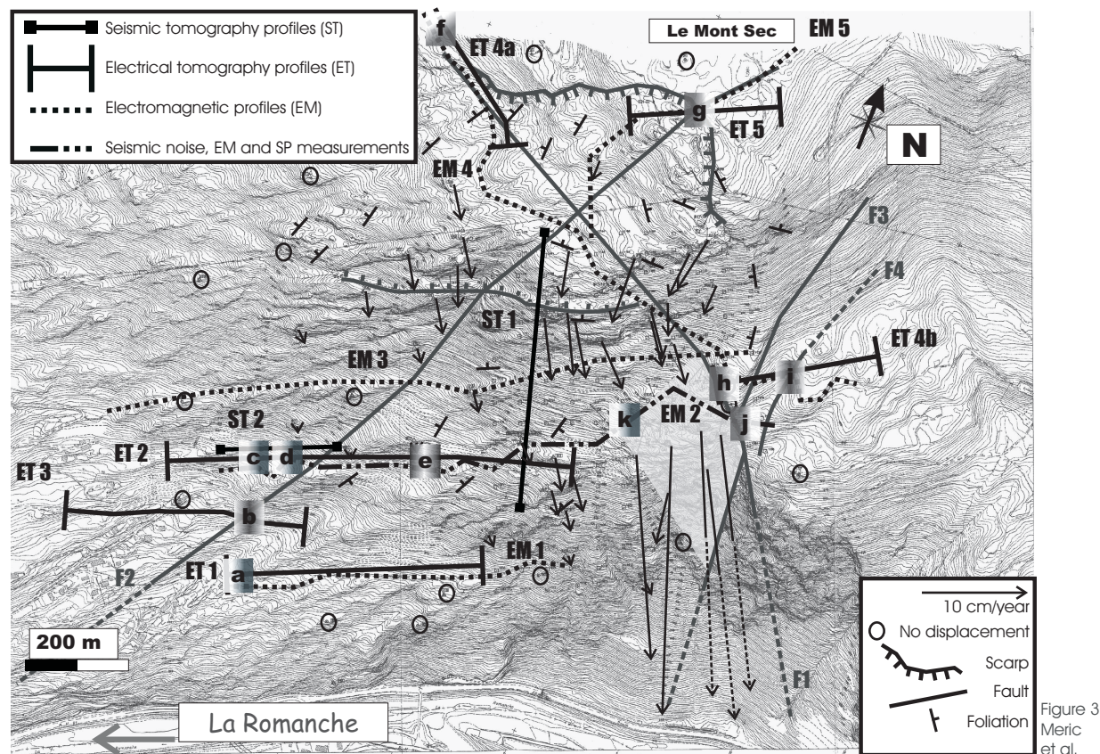
FIG. 4.3 – Topographical map with the main geological structures and displacement rate affecting the Séchillienne hill. The high motion zone is shaded in grey. This map shows also the location of the geophysical profiles (EM : Electromagnetic profiles, ET : Electrical tomography, ST : Seismic tomography). Three geophysical measurement types (electromagnetic, seismic noise and spontaneous potential) were measured along the EM2 profile. Finally this map outlines the main electrical contrasts evinced by the survey and their relation with morphological features. Electrical contrasts are located by boxes the resistive part of which is darker. f and g : Mont Sec scarp ; h and j are eastern limits ; k is a limit inside the movement which delineates the most active part ; b and i are located on faults F2 and F4, respectively ; a, c, d and e are deduced from geophysical prospecting.
