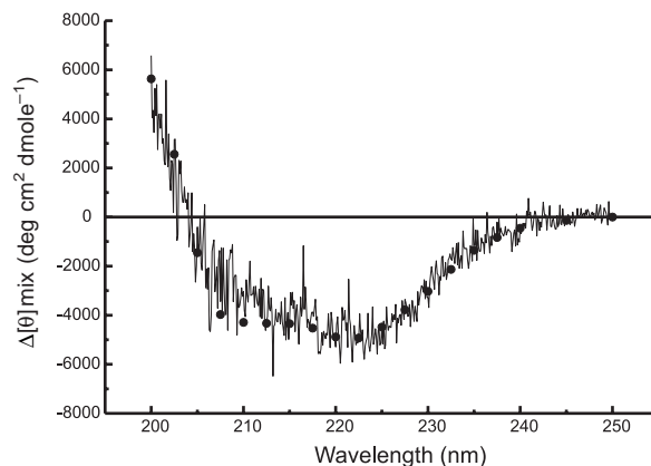
Fig. 6 CD difference spectrum between an equimolar mixture of \alpha_1 and \beta_1 fragments (at a total concentration of 8.7 \mu M) and the sum of the separate components before mixing. The points are calculated for the transition of 14 residues from random coil to \alpha -helix
