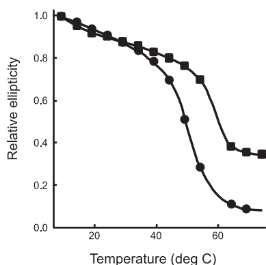
Fig. 3 Thermal denaturation profiles of spectrin \alpha - and \beta -chain fragments, measured by the circular dichroism (CD) change at 222 nm: \alpha_1 (●) and \beta_s (■)
