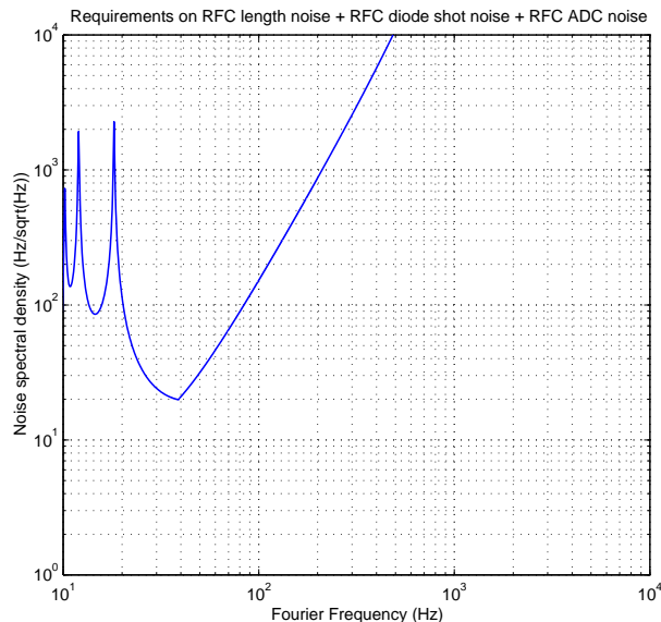
Figure 13: Requirements on the reference cavity length noise
