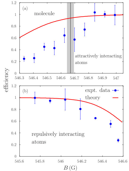
FIG. 5. (Color online) Transfer efficiency of rf association as observed in the experiment and estimated from a Rabi model, both for (a) attractively interacting atoms and molecules and for (b) repulsively interacting pairs. The experimental data contain a global factor which has been chosen such that the value of the outermost right (a) [left (b)] data point is one (see text). Experimental data of (a) from Ref. [9].
