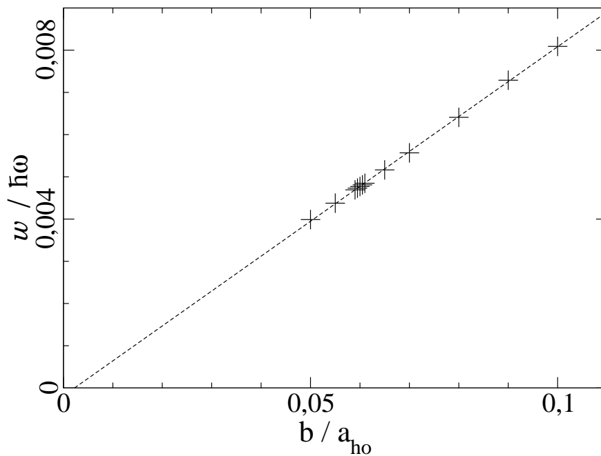
FIG. 3.11 – Coupling w = \langle u | H_{sep} | e \rangle between universal and efimovian state. Remarkably, w is nearly proportional to the range b . The dashed line is a linear fit to the data [ w / (\hbar\omega) = 0.08266 (b / a_{ho}) - 0.000185 ].
