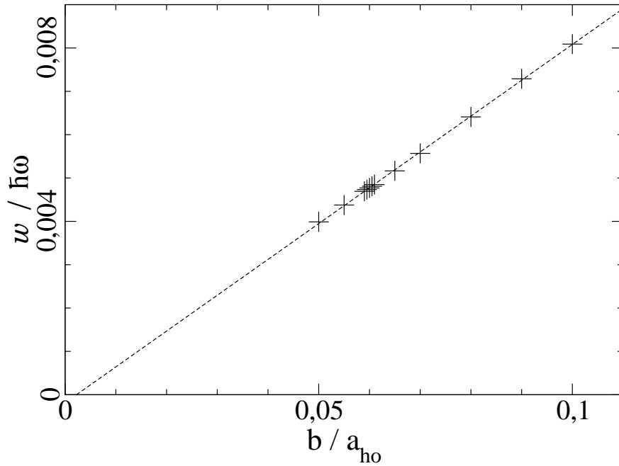
FIG. 3.11 – Coupling w = \langle u|H_{\text{sep}}|e\rangle between universal and efimovian state. Remarkably, w is nearly proportional to the range b . The dashed line is a linear fit to the data [ w/(\hbar\omega) = 0.08266(b/a_{\text{ho}}) - 0.000185 ].
