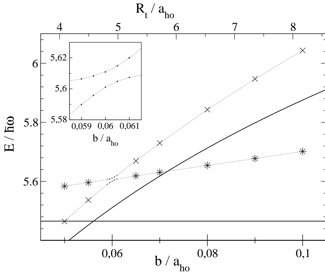
FIG. 3.7 – Within the zero-range model, there is a crossing between universal and efimovian states (solid lines). This becomes an avoided crossing for the separable potential model (dotted lines). [Moreover there is a small shift between the two models due to finite-range corrections; for the universal state, this correction agrees with the effective range model as shown in Fig. 3.5, the stars on Fig. 3.5 representing the same universal states as on the present Figure.]
