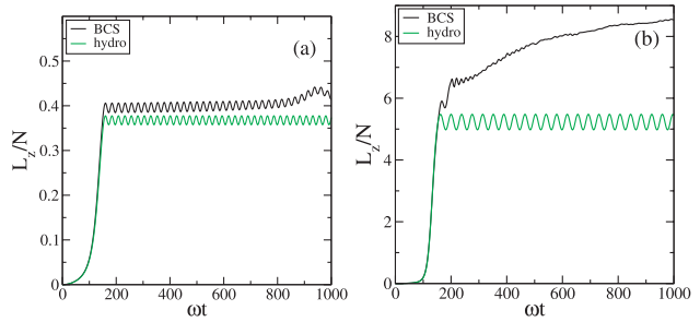
Fig. 6. Angular momentum per particle in the gas, in units of \hbar , as a function of time, for a final rotation frequency (a) \Omega = 0.6\omega and (b) \Omega = 0.8\omega . Black curves: numerical simulations of the 2D time dependent BCS equations on a 64 \times 64 grid. Green curves (color online): time dependent superfluid hydrodynamic theory of Section 2 [solution of Eqs. (12, 13) with a time dependent quadratic ansatz].
