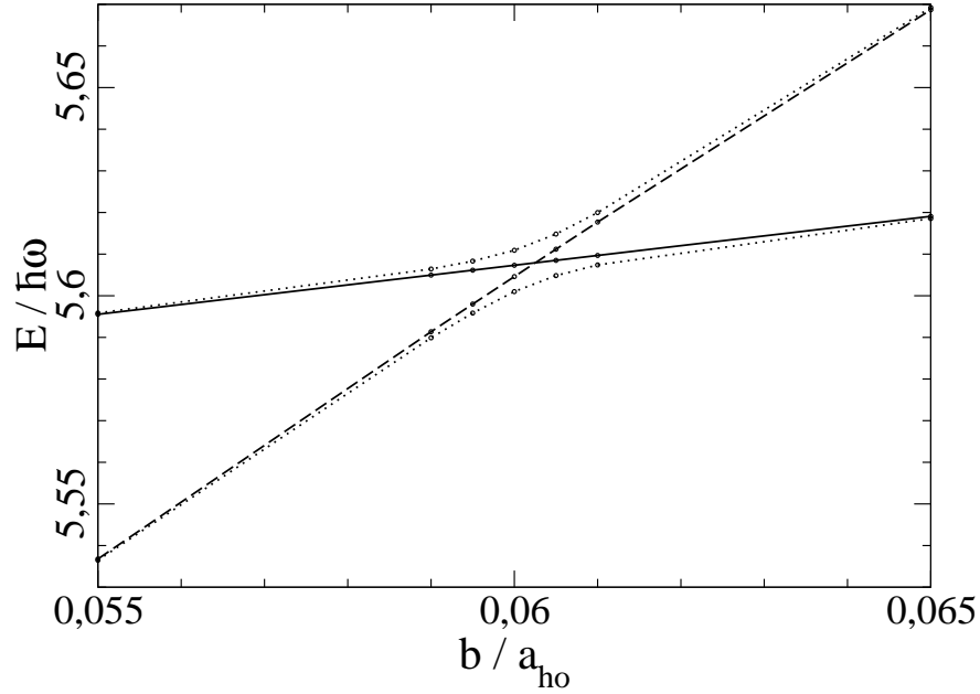
FIG. 3.10 – The diagonal matrix elements E_e^0 = \langle e|H_{\text{sep}}|e\rangle (dashed line) and E_u^0 = \langle u|H_{\text{sep}}|u\rangle (continuous line) of H_{\text{sep}} simply cross, while the eigenvalues E_1 and E_2 of H_{\text{sep}} have an avoided crossing (dotted lines).
