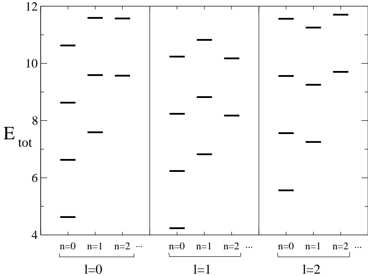
FIG. 3.3 – The spectrum for 3 fermions (in units of \hbar\omega ) is formed of ladders with energy steps 2 : E = s_{l,n} + 1 + 2q, q \in \mathbb{N} . Here we assume that the center of mass is in its ground state so that the total energy is E_{\text{tot}} = E + 3/2 . l is the total angular momentum of the system. The values of s are known by numerical solution of the transcendental equation Eq. (3.39), cf. Tab. 3.1 and Fig. 3.2. The ground state has an angular momentum l = 1 and an energy E_{\text{tot}} \simeq 4.27 . The eigenstates in common with the non-interacting problem (Sec. 3.1.e) are not represented.
