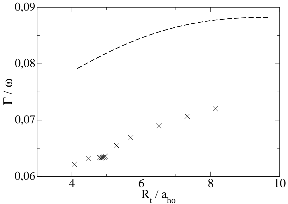
FIG. 3.8 – Loss rate of the efimovian state as a function of the 3-body parameter. Dashed line : analytical prediction of the zero-range Braaten-Hammer approach [Eq. (3.131) p. 103], with the parameter \eta_* = 0.06 extracted from the Cesium experiment [2]. Crosses : numerical result of the separable-potential-base effective Hamiltonian, with the parameter B_3 = 25 extracted from the same experiment.
