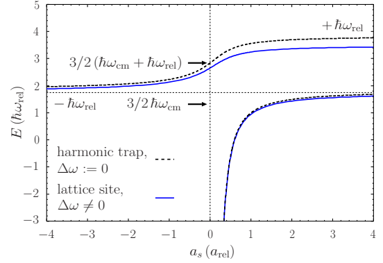
FIG. 1. (Color online) Energy eigenvalues of ^{40}\text{K} and ^{87}\text{Rb} as a function of scattering length without (black dashed line) and with coupling terms (blue solid line) due to anharmonicity and unequal trap frequencies in the lattice for parameters: V_{\text{Rb}}=40.5E_{r,\text{Rb}} , V_{\text{K}}=0.86V_{\text{Rb}} , and \lambda=1030 nm. The deviation between the idealized model and the full solution is substantial in particular for the upper branch.
