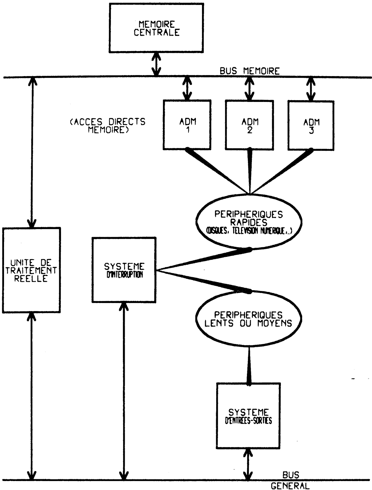
Figure 9: ARCHITECTURE DU T1600
