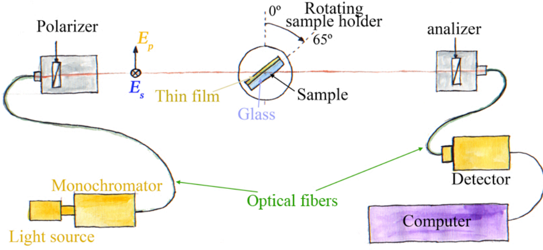
Figure 6.1: Scheme of the experimental setup used for extinction measurements. The letters p and s in the scheme correspond to the p- and s-polarization of the incident electric field, respectively.
