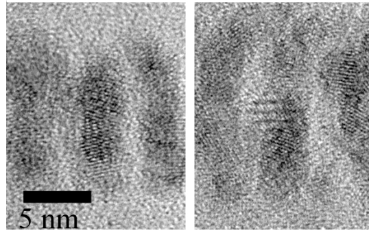
Figure 7.12: Cross-section TEM images of NCl thin films produced with (left) X_{25} and (right) X_{30} .
