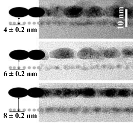
Figure 3.5: Cross-section TEM images. From top to bottom the images correspond to X = 4.0, 6.0 and 8.0 nm (The error is estimated to be \Delta X \pm 0.2 nm).
