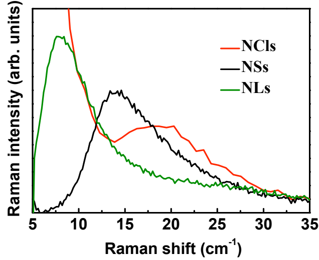
Figure 7.6: Experimental Stokes Raman spectra of Ag NCIs, NSs, and NLs excited at 413 nm (NCIs and NSs) and 514 nm (NLs). The incident laser beam was p-polarized and the polarization of the scattered light was not analyzed.
