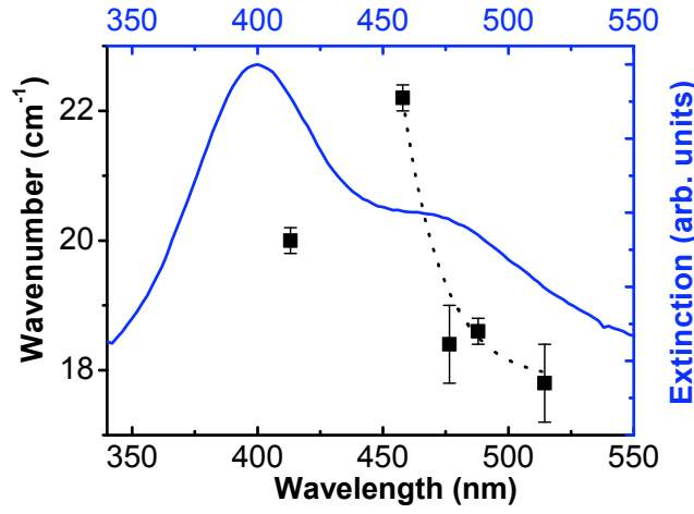
Figure 8.1: (Filled squares) Experimental frequencies of the vibrations of the NCLs versus excitation wavelength. The laser beam was p-polarized, and the polarization of the scattered light was not analyzed. The dotted line is a guide to the eye. (blue) Experimental extinction spectrum of the NCLs, recorded using p-polarized light and an angle of incidence of 65^\circ .
