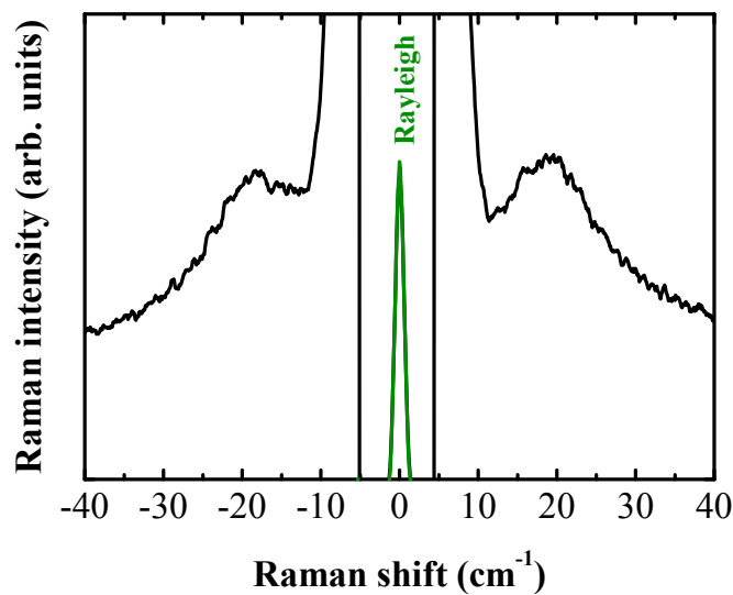
Figure 6.6: Experimental Stokes and anti-Stokes room temperature Raman spectrum of Ag NCl s excited at 488 nm. The incident laser beam was p-polarized and the polarization of the scattered beam was not analyzed.
