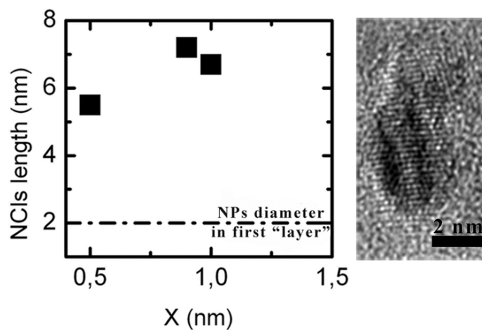
Figure 3.7: Height, H , of NCLs as a function of the effective thickness of the matrix layer X and cross-section HREM image of one of the NCLs produced with X=D .
