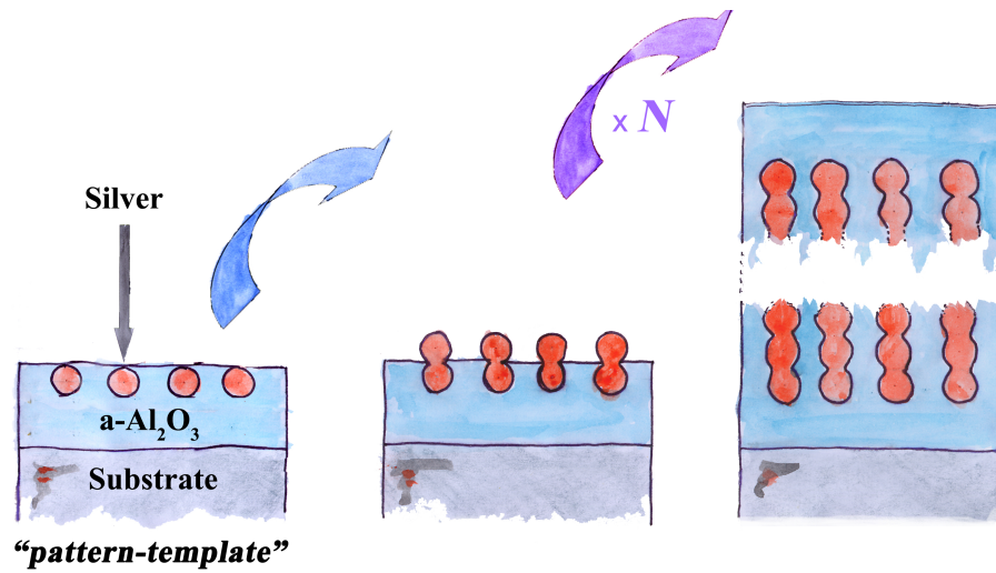
Figure 2.7: Schematic for the production of Ag NCLs
