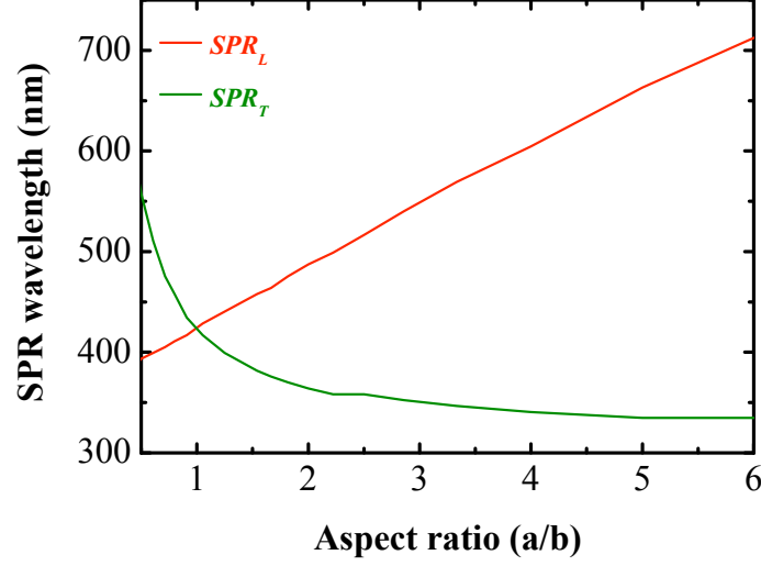
Figure 5.10: Calculated position of the transverse, SPR_T , and longitudinal, SPR_L , SPRs of a Ag ellipsoidal NP embedded in \alpha - Al_2O_3 as a function of the aspect ratio a/b
