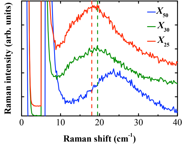
Figure 7.14: Experimental Stokes Raman spectra of samples containing Ag NCl produced with decreasing X . The incident laser beam was p-polarized and the polarization of the scattered light was not analyzed. Dashed lines are only guides for the eyes.
