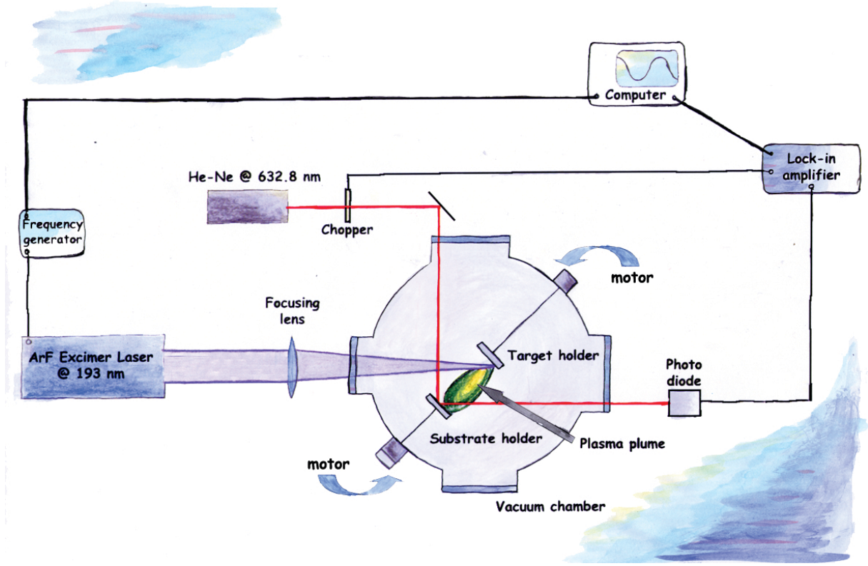
Figure 1.7: PLD experimental setup
