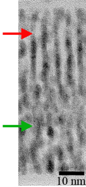
Figure 7.10: Cross-section TEM image of the sample N = 50 . The red arrow shows discontinuities while the green one shows misalignment of NCLs.
