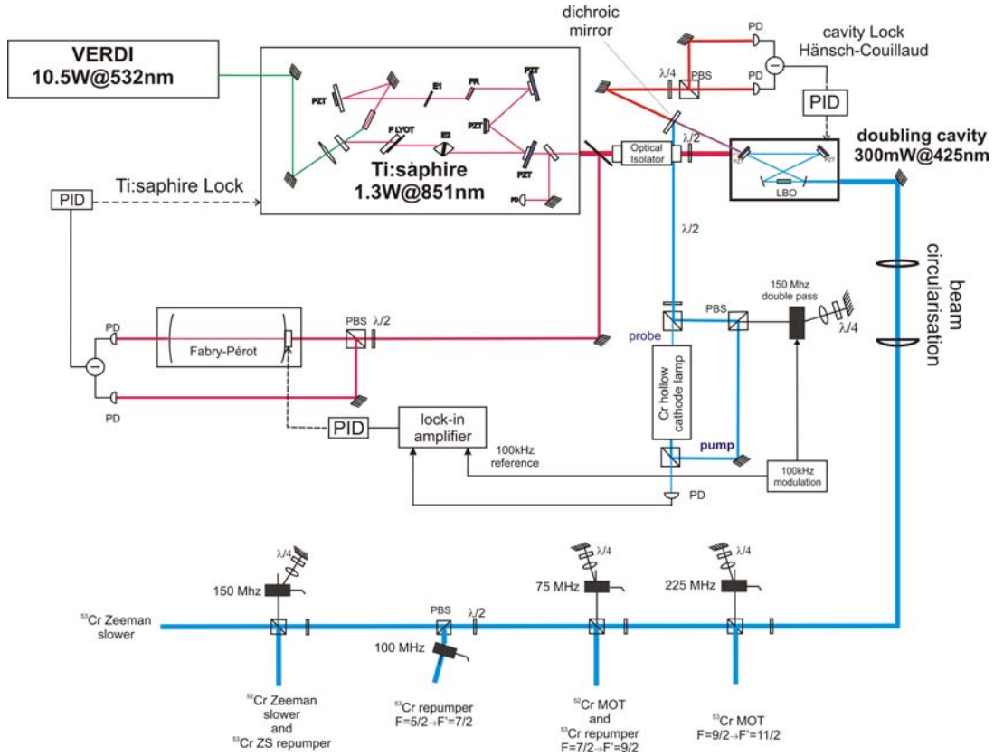
Figure 2.6: Scheme of the laser system for magneto-optically trapping and cooling Cr atoms.
