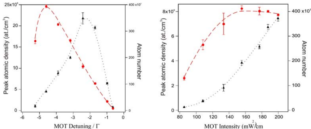
Figure 3.16: A) ^{53}\text{Cr} MOT atom number (dots) and peak atom density (triangles) as a function of the normalized detuning of the MOT beams, for a total laser intensity of 200 mW/cm 2 B) Atom number (dots) and peak atom density (triangles) as a function of the total power in the MOT cooling beams, for a detuning of -21.5 MHz.
