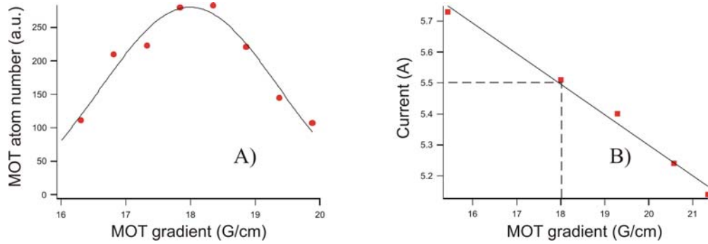
Figure 3.3: A): 52 Cr MOT atom number as a function of the magnetic field gradient. The optimal gradient value is 18 G/cm. B): Value of the current of the ZS extraction coil, obtained by optimizing the MOT atom number, as a function of the MOT gradient.
