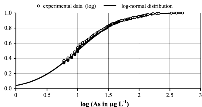
Fig. 3. Distribution of logarithmic As concentrations compared to a normal distribution. The mean value is estimated from the logarithm of the median concentration ( 10 \mu\text{g L}^{-1} ) and the variance from the set of measurements greater than the median.
