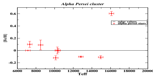
Fig. 1- Abundance of iron versus the effective temperature
