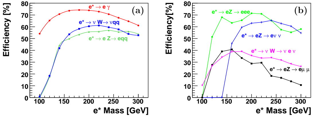
Figure 5.32: Efficiency to select e^* events in each decay channel: for three main decay channels (a): e^* \rightarrow e\gamma , e^* \rightarrow \nu W \rightarrow \nu qq and e^* \rightarrow eZ \rightarrow eqq ; for the leptonic decay channels of the Z or W boson (b): e^* \rightarrow eZ \rightarrow \mu\mu , e^* \rightarrow eZ \rightarrow ee and e^* \rightarrow \nu W \rightarrow \nu e\nu , e^* \rightarrow eZ \rightarrow \nu\nu .
