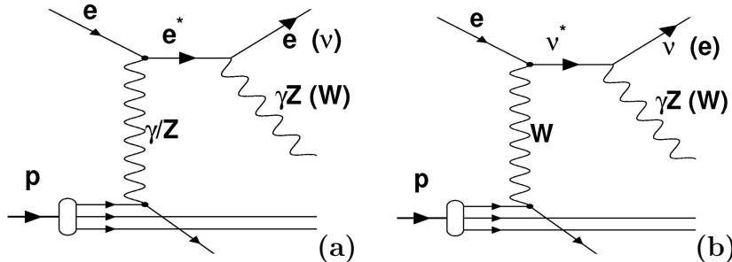
Figure 2.14: Diagrams of the production of excited electrons (a) and excited neutrinos (b).
