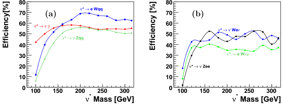
Figure 6.32: Efficiency to select \nu^* events in each decay channel for the three main decay channel in (a): \nu^* \rightarrow \nu\gamma , \nu^* \rightarrow eW \rightarrow qq and \nu^* \rightarrow \nu Z \rightarrow qq decay channel; for the leptonic decay channels of the Z or W bosons in (b): \nu^* \rightarrow \nu Z \rightarrow ee , \nu^* \rightarrow eW \rightarrow e\nu and \nu^* \rightarrow eW \rightarrow \mu\nu .
