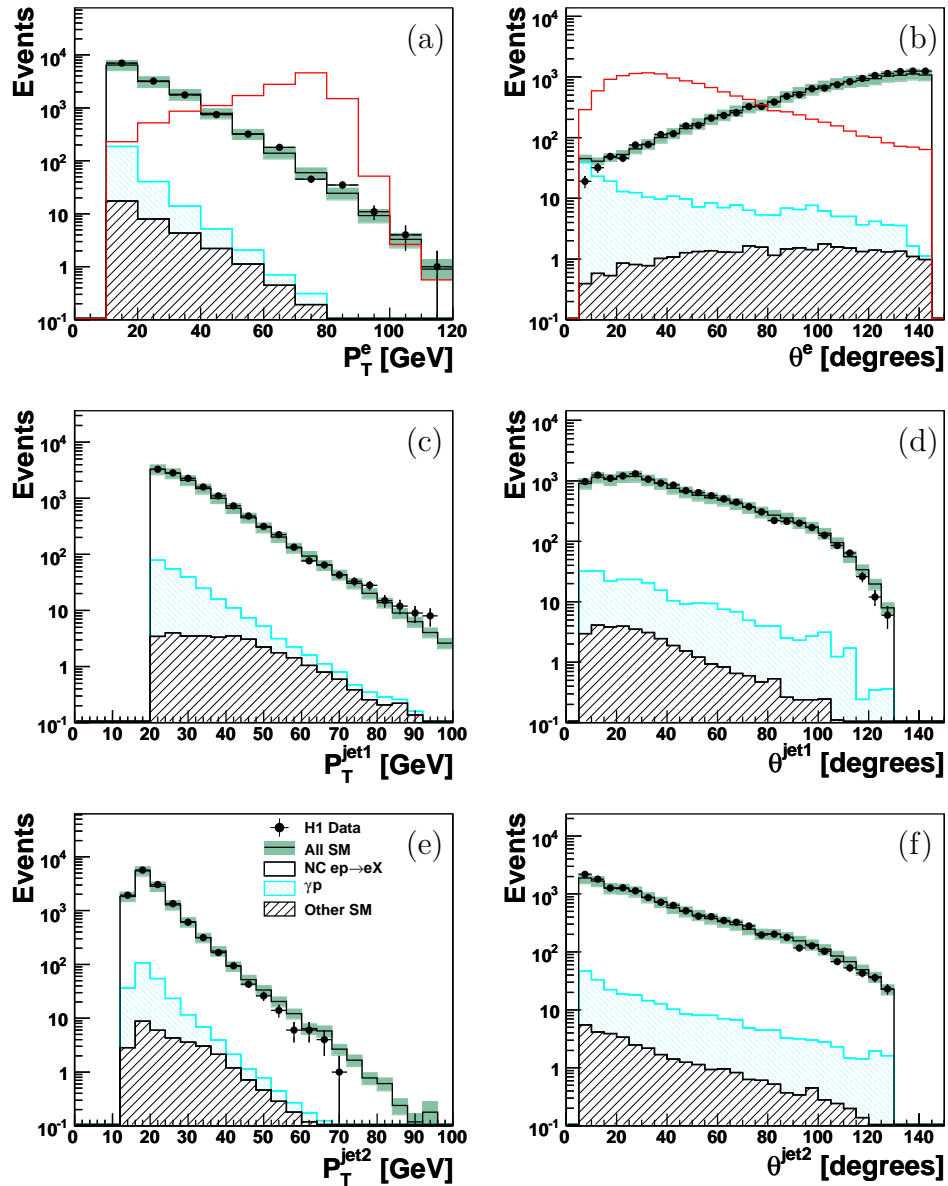
Figure 5.10: Transverse momentum (a) and polar angle (b) distributions of the electron in NC DIS events with at least two high P_T jets. Transverse momentum (c,e) and polar angle (d,f) distributions of the two jets associated to the decay of a Z candidate boson. The red line in (a,b) corresponds to the e^* signal at M_{e^*} = 200 GeV.
