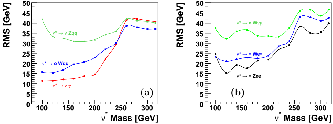
Figure 6.33: Width of the reconstructed \nu^* masses as a function of the excited neutrino generated mass: for the three main decay channels (a): \nu^* \rightarrow \nu\gamma , \nu^* \rightarrow eW \rightarrow qq , \nu^* \rightarrow \nu Z \rightarrow qq (red, blue and green curves); for the leptonic decay channels of the Z and W boson: \nu^* \rightarrow \nu Z \rightarrow ee , \nu^* \rightarrow eW \rightarrow e\nu and \nu^* \rightarrow eW \rightarrow \mu\nu .
